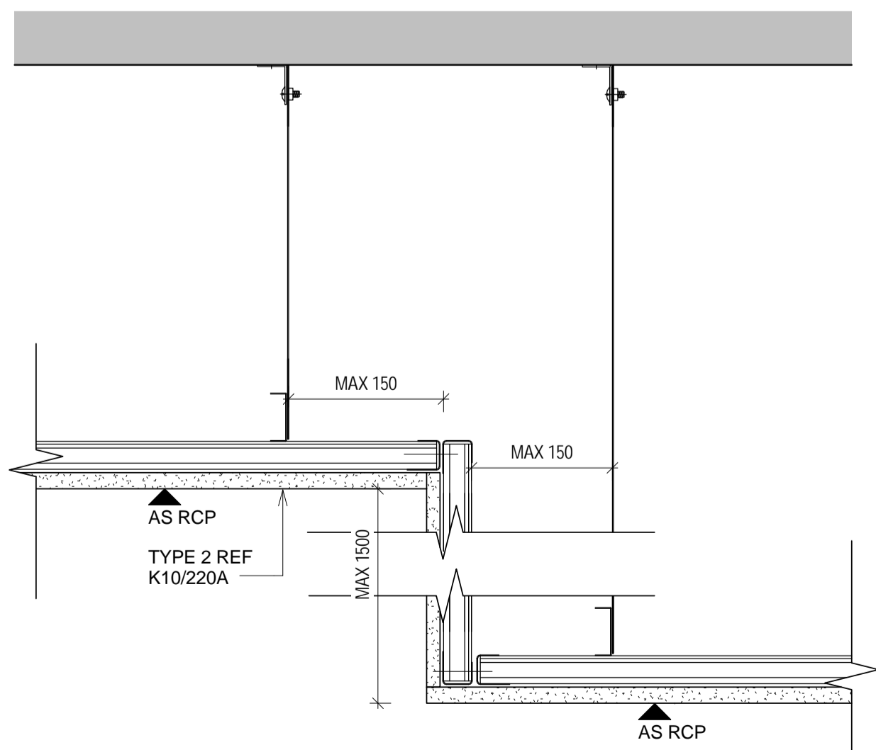
8 TYPE 2 DETAIL CHANGE OF LEVEL 1:5
