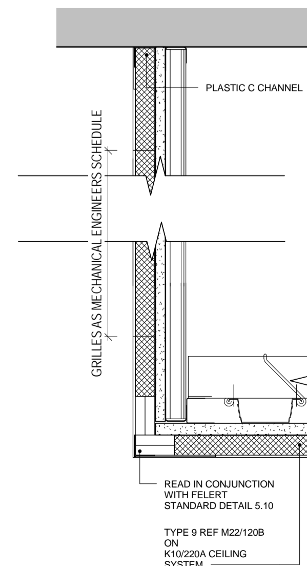
10 TYPE 9 BULKHEAD ACCESS PANEL DETAIL 1:5
