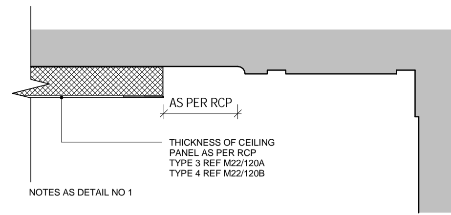
2 TYPE 3 / TYPE 4 CORNICE DETAIL 1:5
