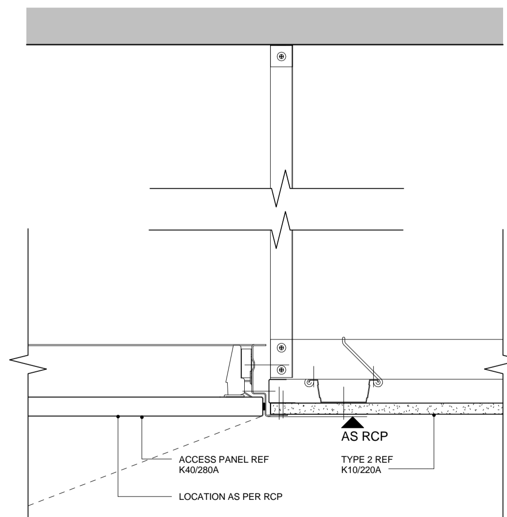
9 TYPE 2 ACCESS PANEL DETAIL 1:5
