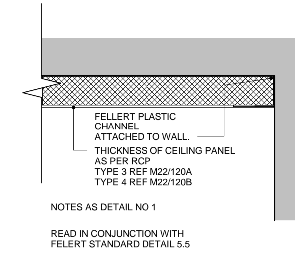
11 TYPE 3 / TYPE 4 DETAIL WITHOUT MARGIN 1:5
