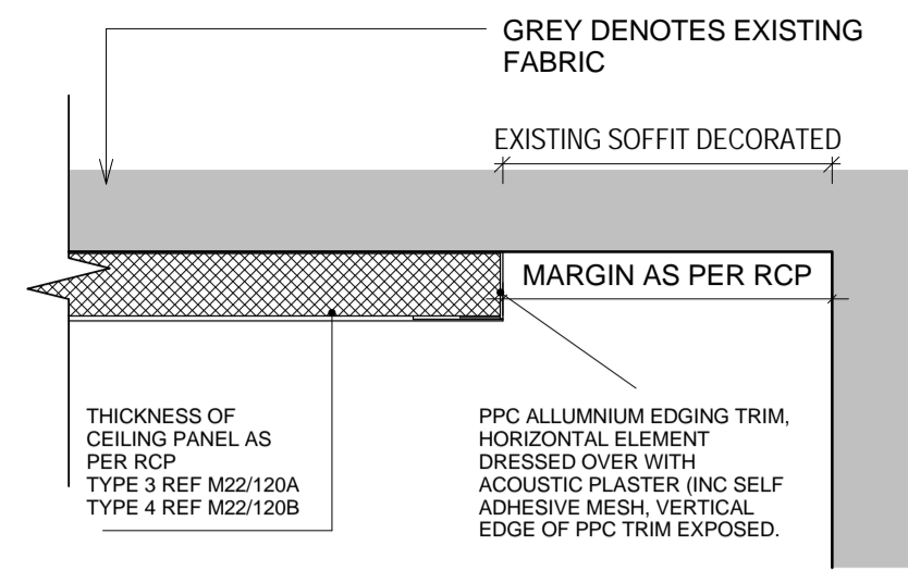
1 TYPE 3 / TYPE 4 DETAIL 1:5
