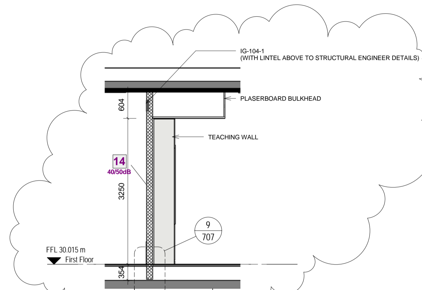
5 1.01 SECTION
