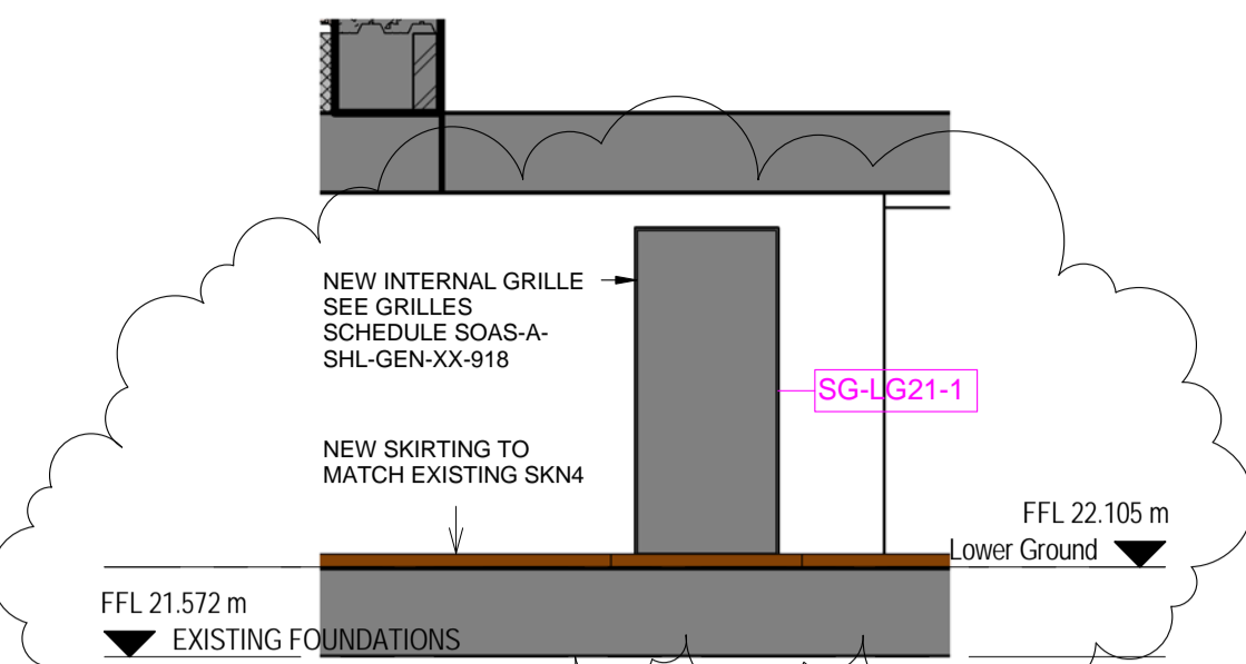
4 LG.29 ELEVATION
