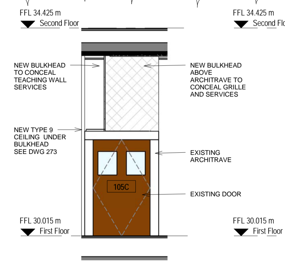
8 1.05 BULKHEAD ELEVATION
