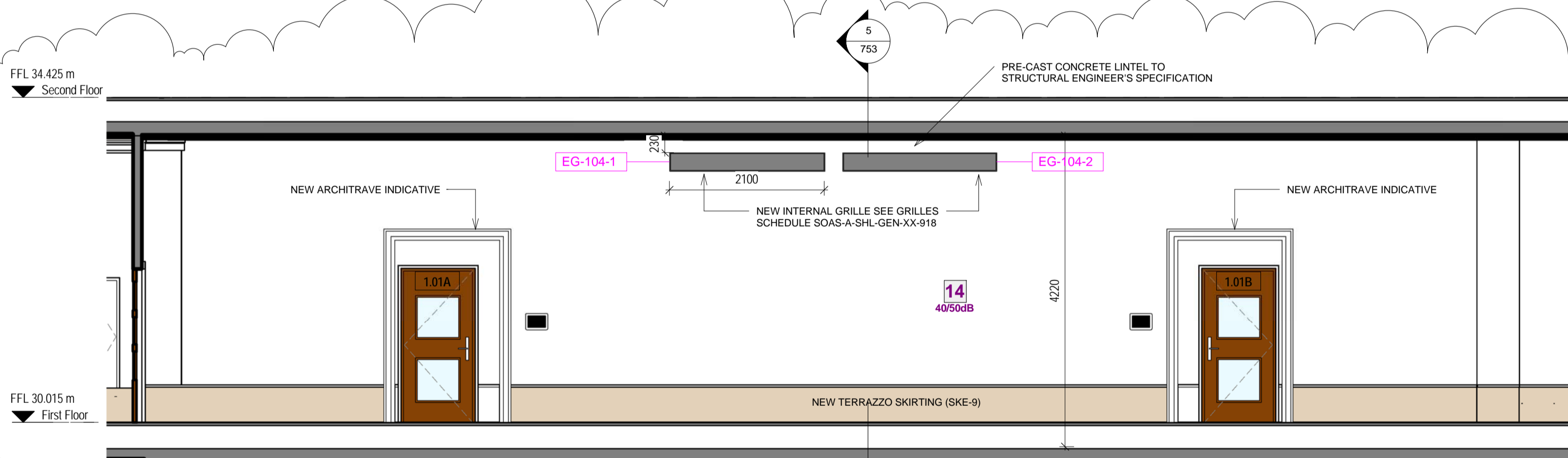
2 1.04 INTERNAL ELEVATION
