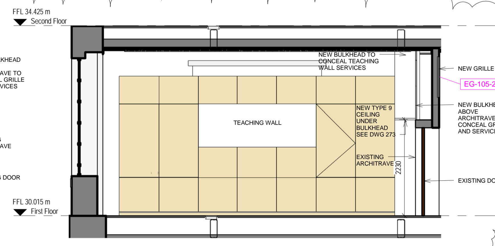
9 1.05 INTERNAL ELEVATION
