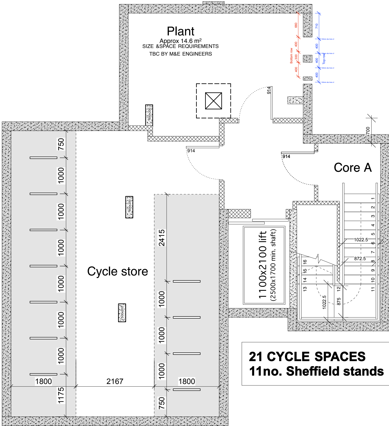
CORE A CYCLE STORAGE DETAIL PLAN 1:50@A1, 1:100@A3
