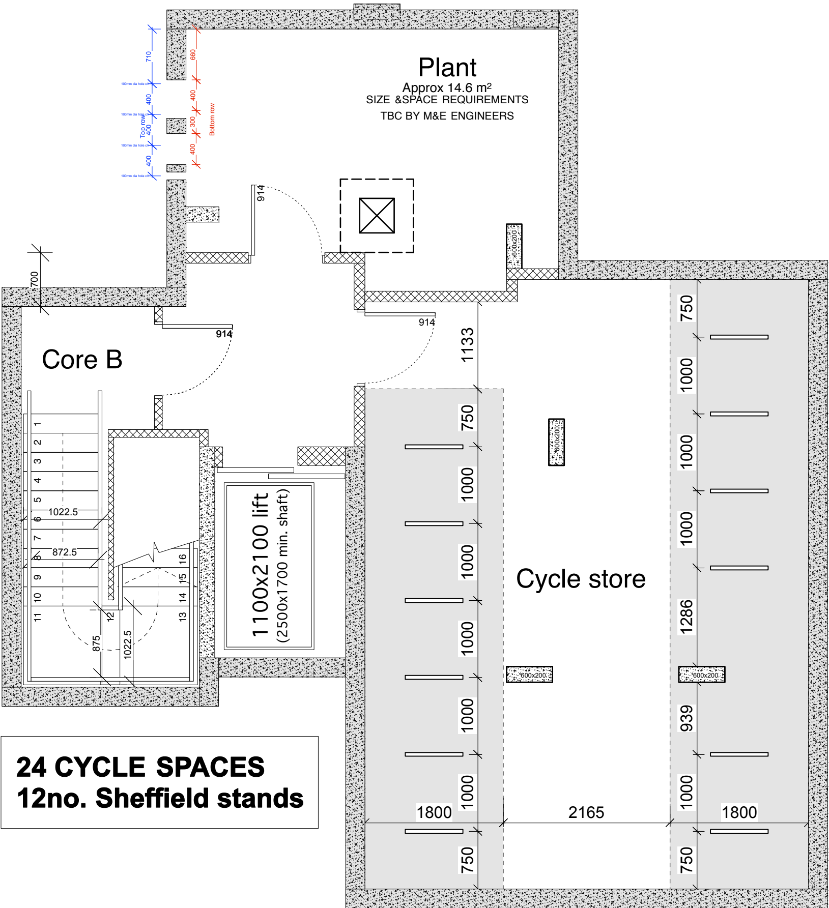
CORE B CYCLE STORAGE DETAIL PLAN 1:50@A1, 1:100@A3
