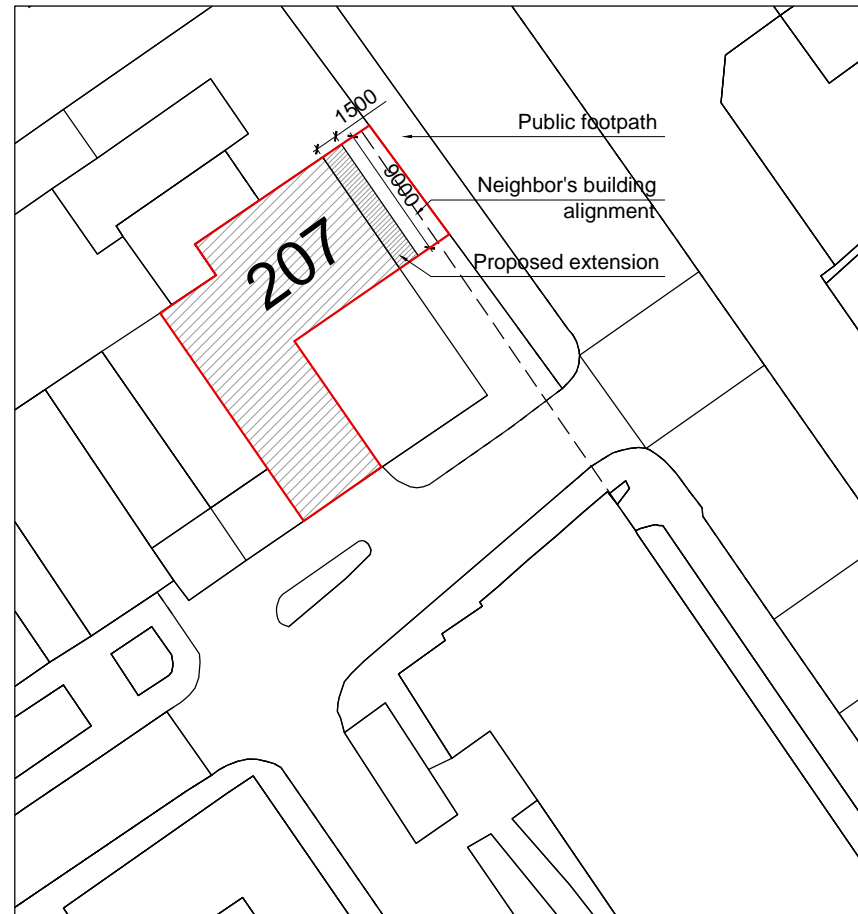
SITE PLAN 0 10 20 30m scale 1:500
