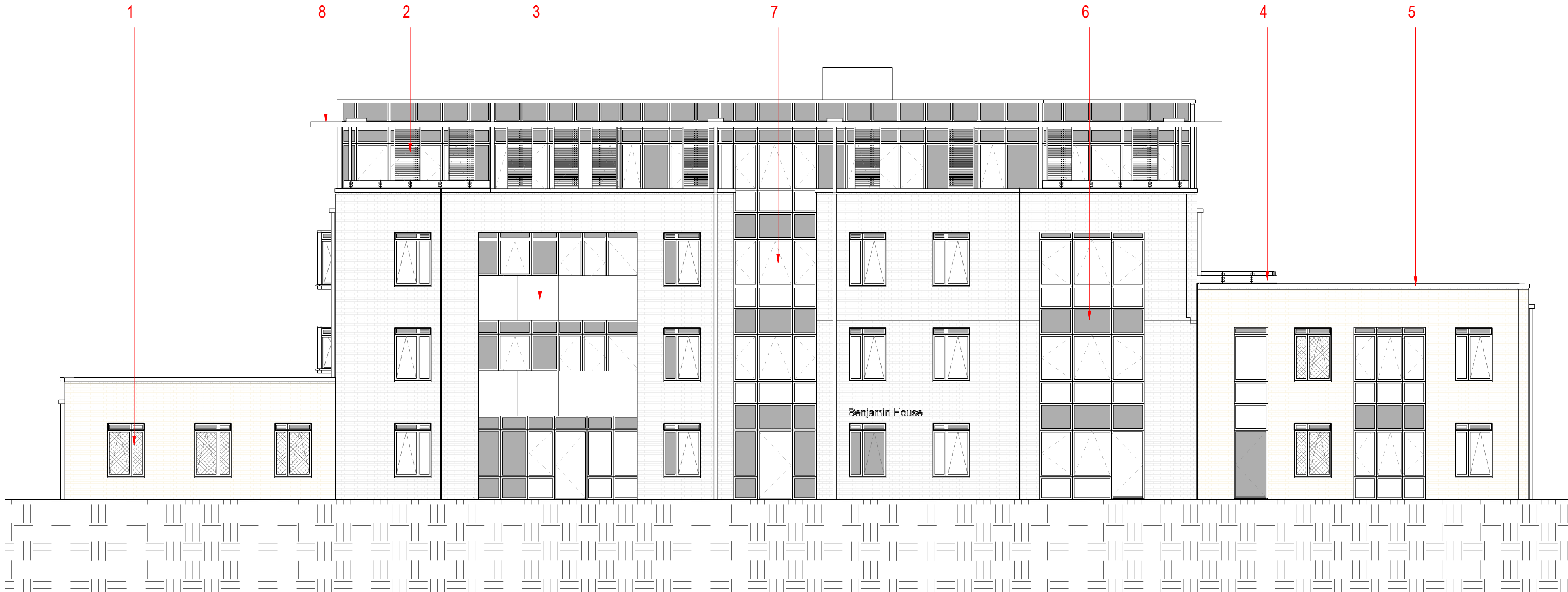
Block B - North East Elevation
