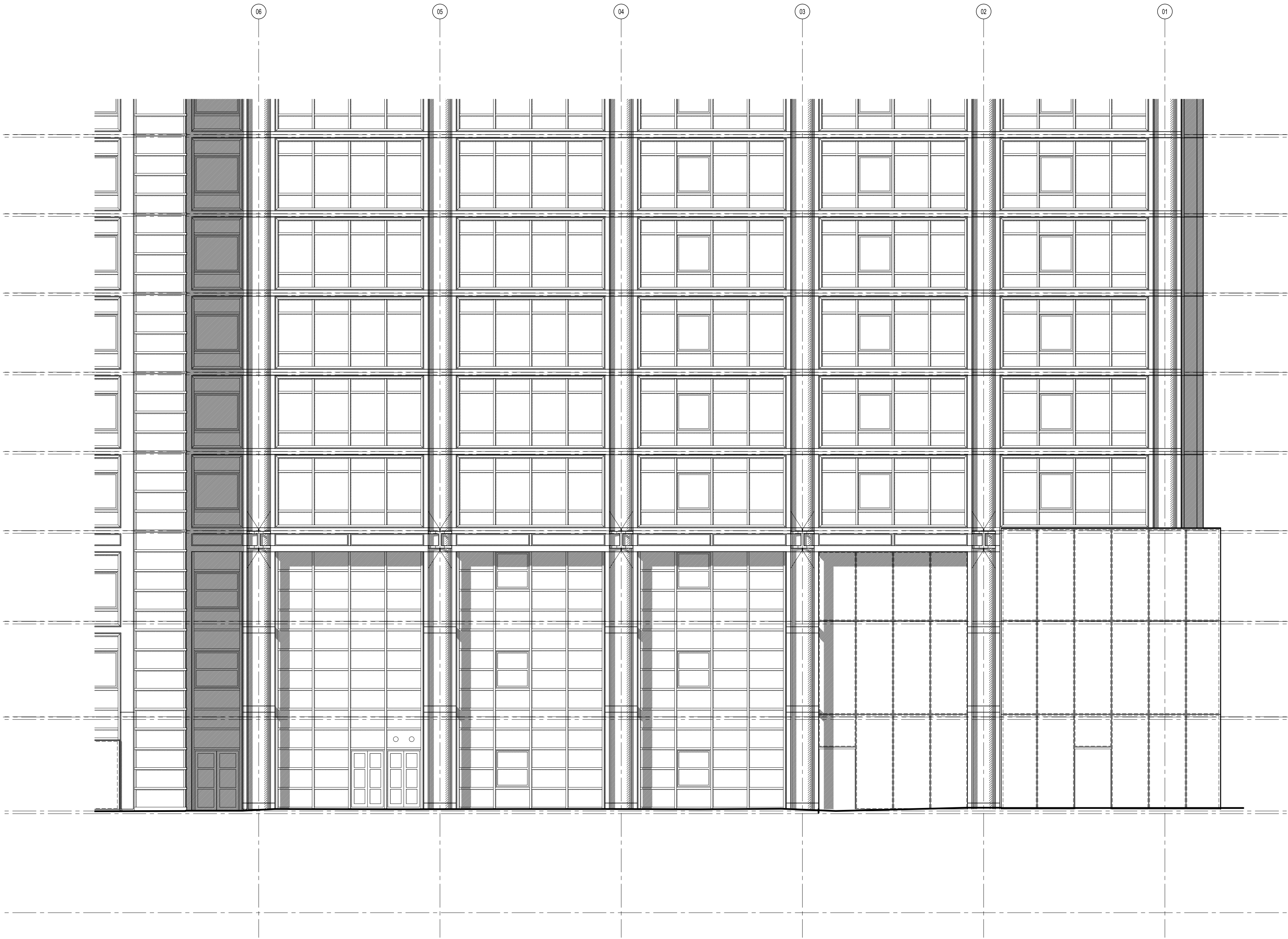
01 EAST ELEVATION 1/100
