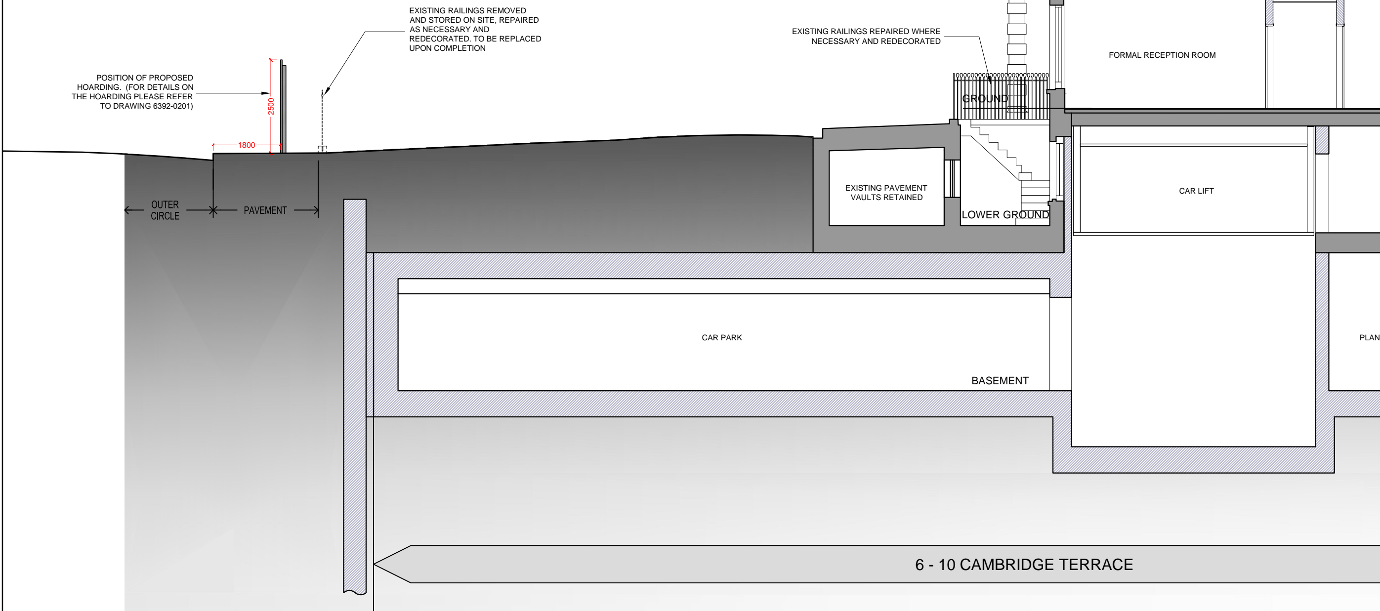
PART SECTION SHOWING HOARDING BOARD IN RELATION TO THE FACADE OF CAMBRIDGE TERRACE
