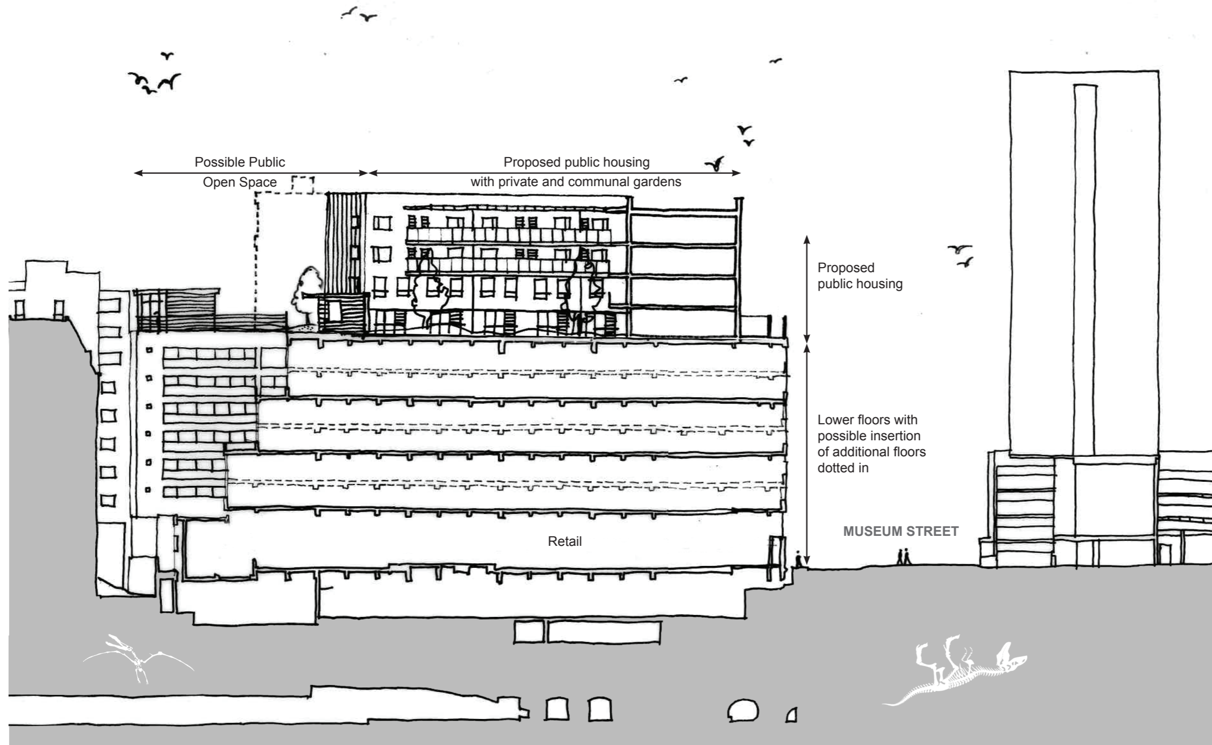
Option 2 Scheme Section Scale 1:400
