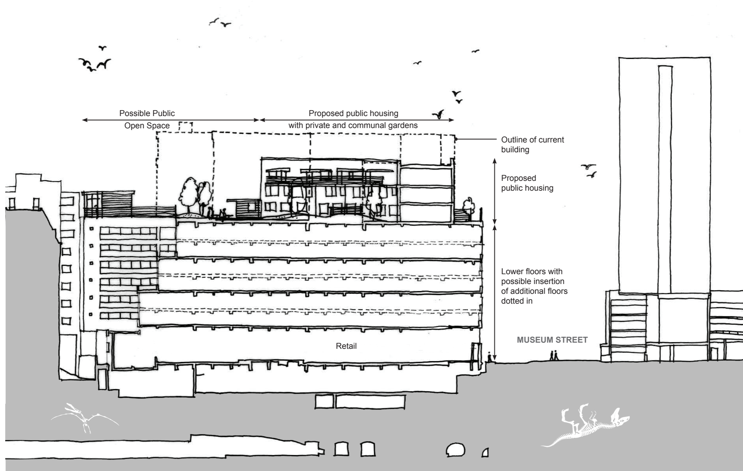
Option 1 Scheme Section Scale 1:400
