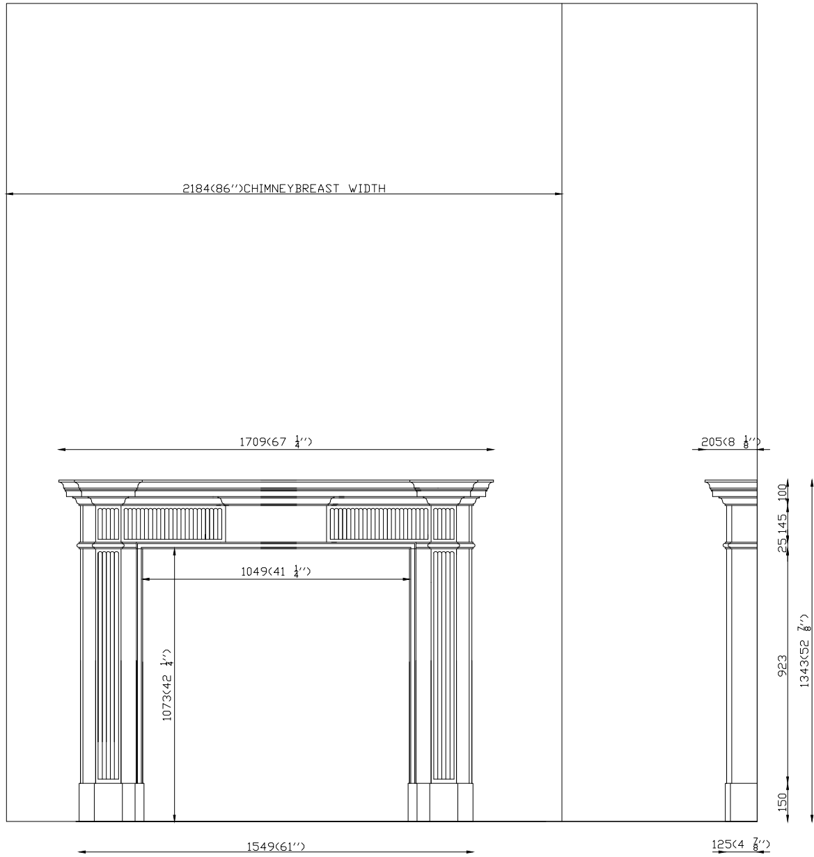
FRONT ELEVATION
