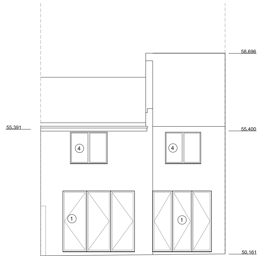
Elevation 4 Proposed
