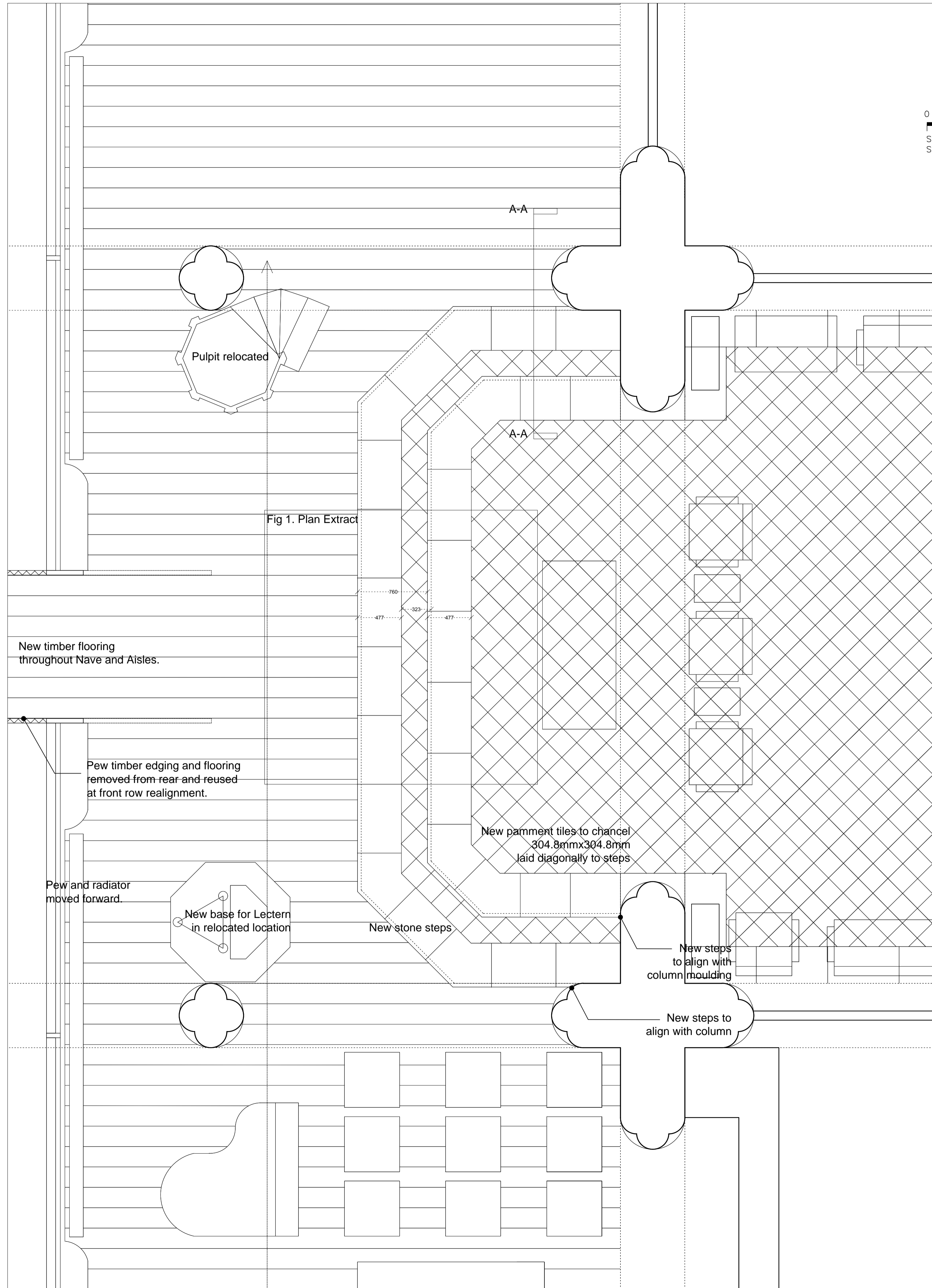
Plan 1:25@A1 / 1:50@A3
