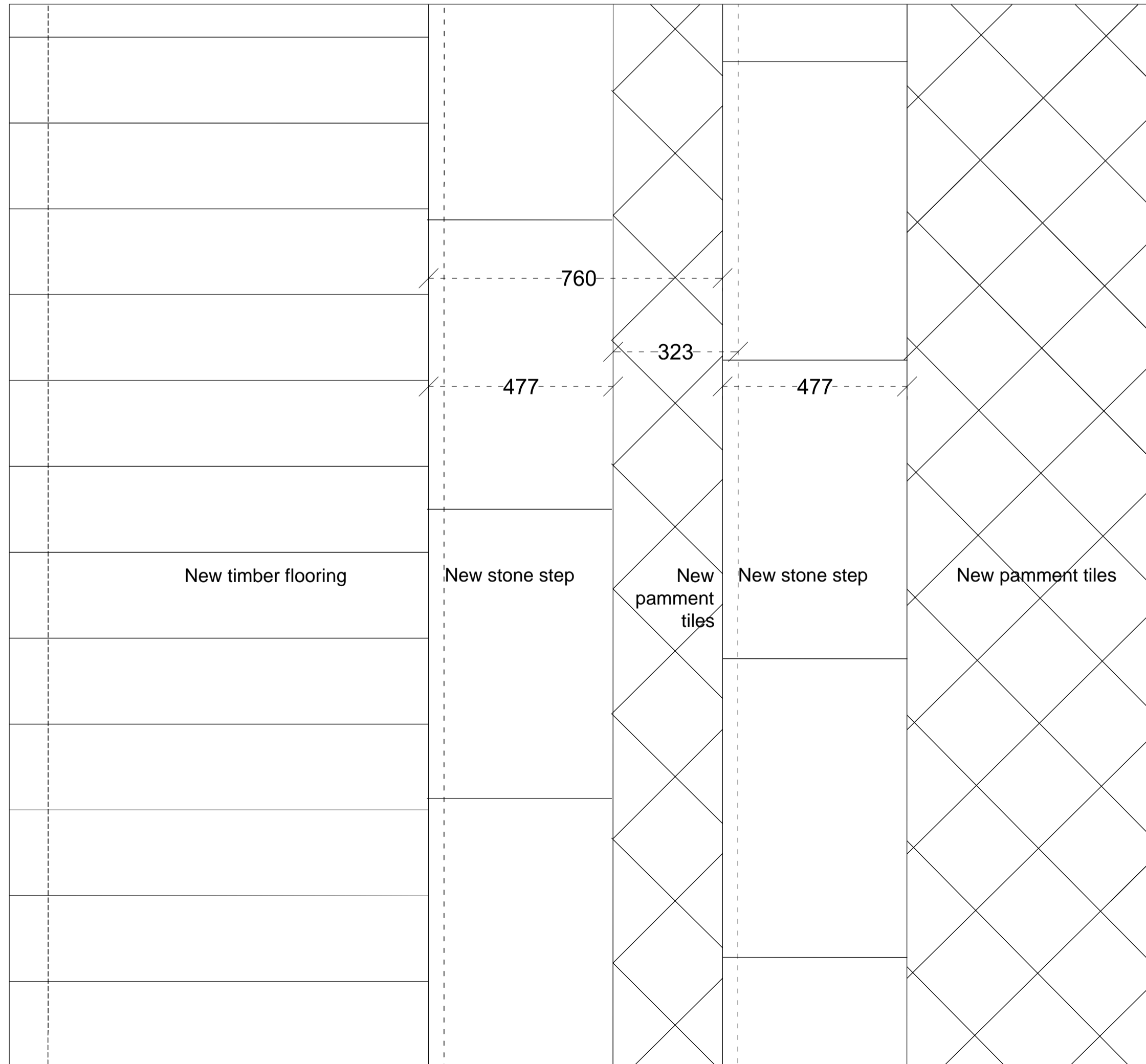
Fig1. Plan Extract 1:10@A1 / 1:20@A3
