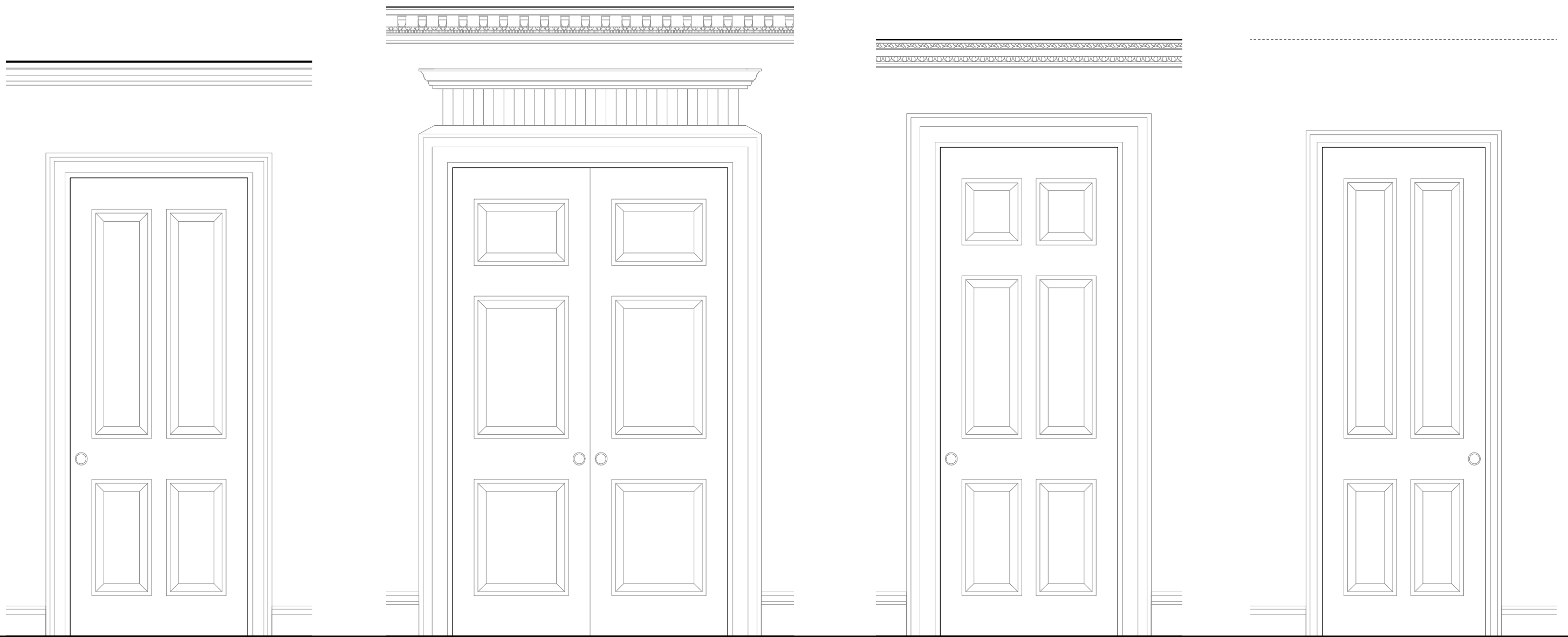
LOWER GROUND FLOOR TYPICAL INTERIOR DETAILS
