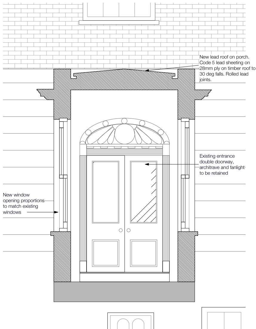
PROPOSED CROSS SECTION
