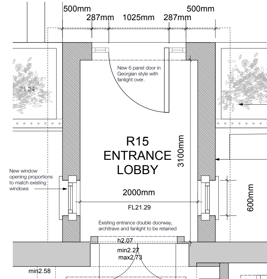
PROPOSED PORCH PLAN
