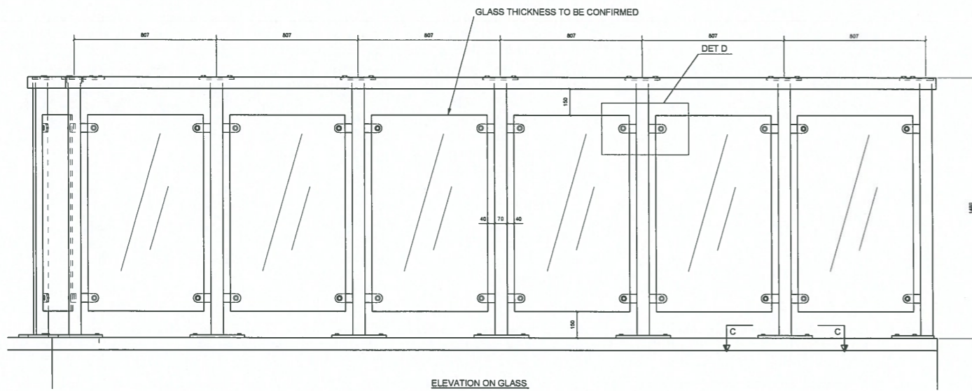
ELEVATION ON GLASS
