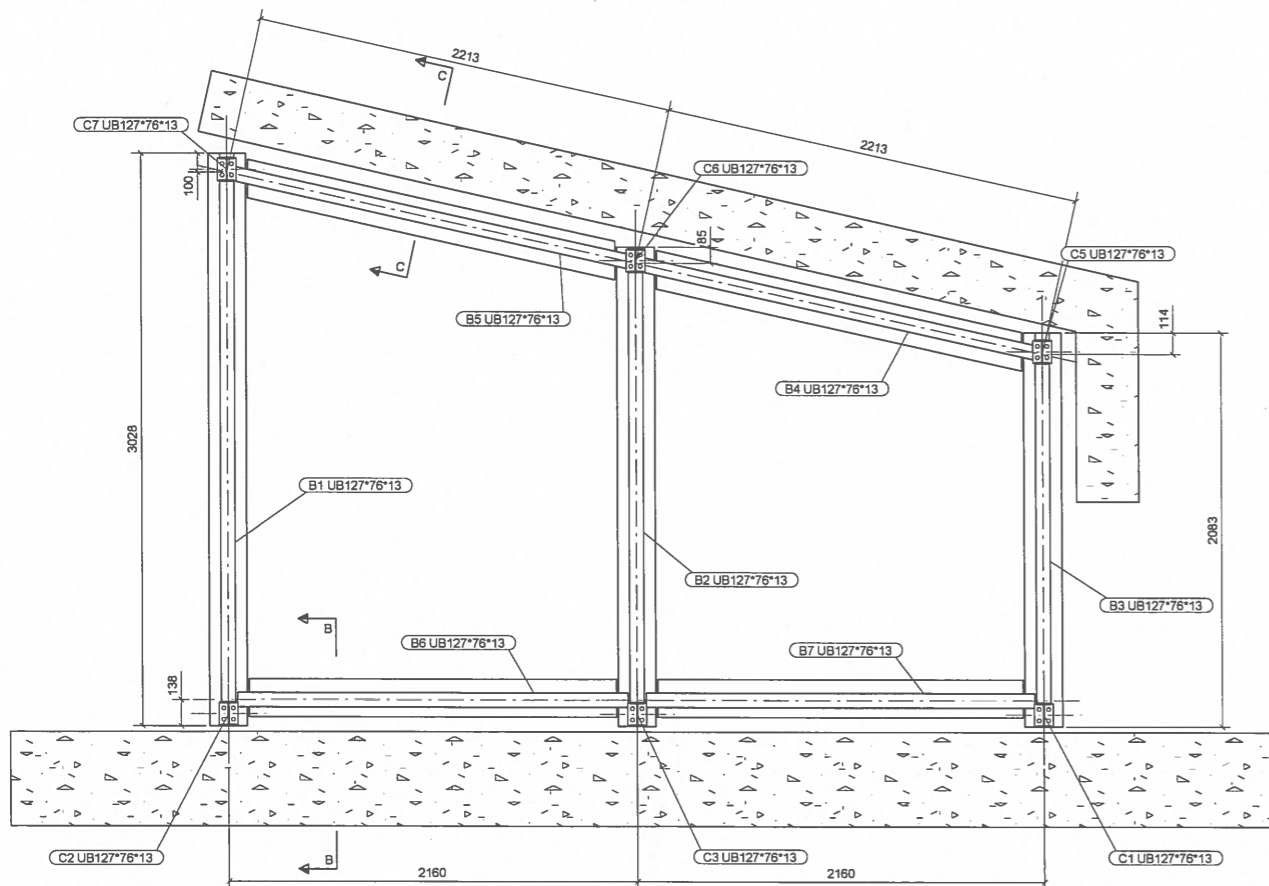
SECTION OF LOWER LEVEL
