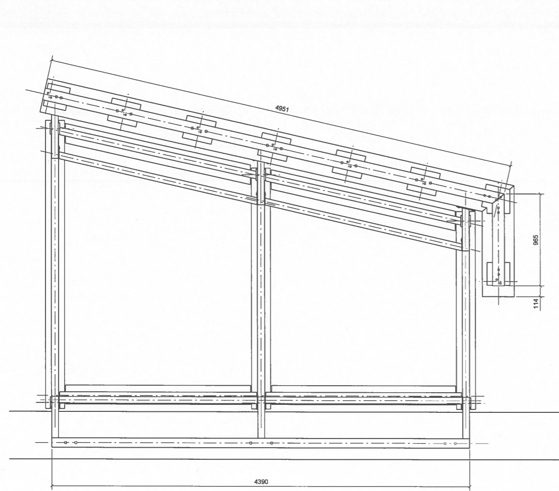
Plan +0
