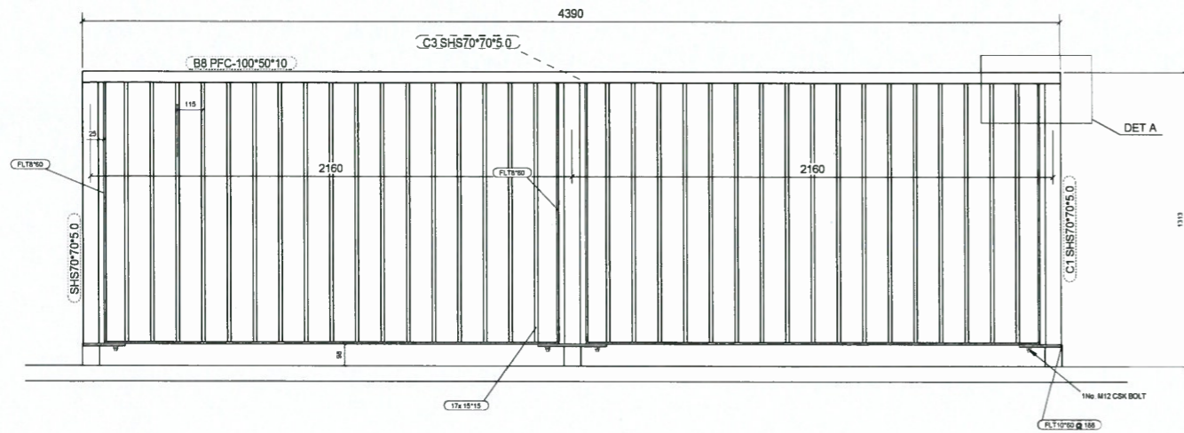
ELEVATION ON GAURD RAIL
