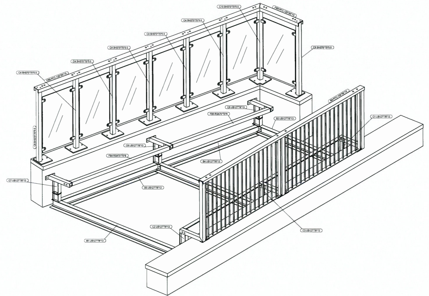
3d - 3d SECTION OF LOWER LEVEL
