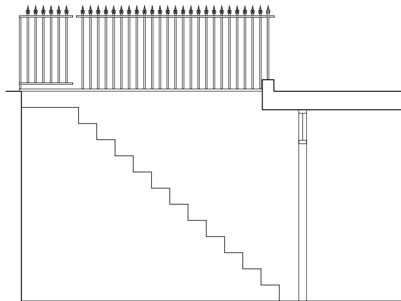
EXISTING SECTION AA (PART OF)
