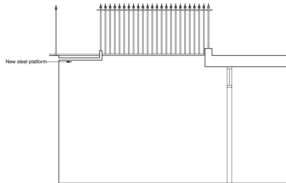
PROPOSED SECTION AA (PART OF)
