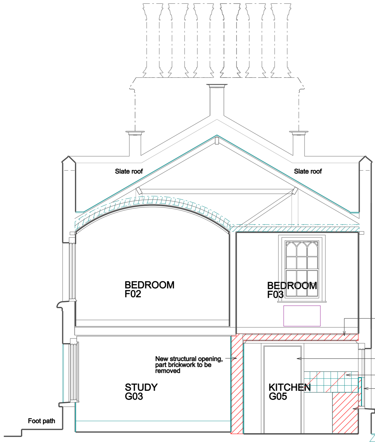
SECTION BB'
