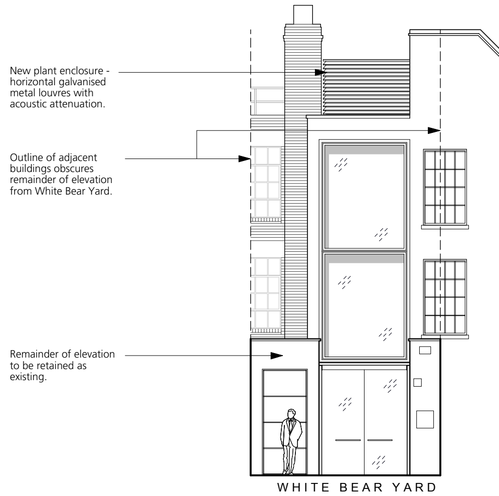
1 White Bear Yard Elevation
