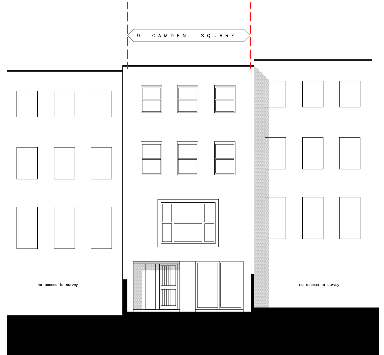
SOUTH EAST ELEVATION
