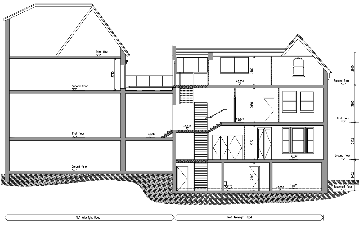
proposed section through A-A
