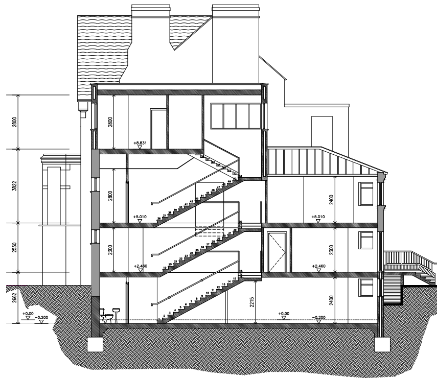
proposed section through B-B
