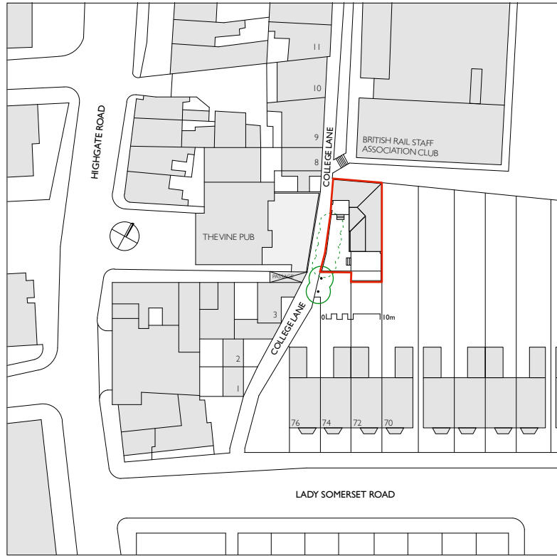
1 : 1000 SITE PLAN AS EXISTING
