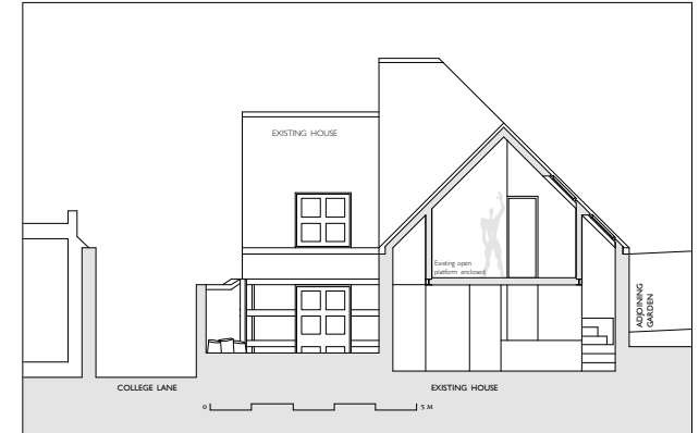
1 : 200 WEST - EAST SECTION AS EXISTING
