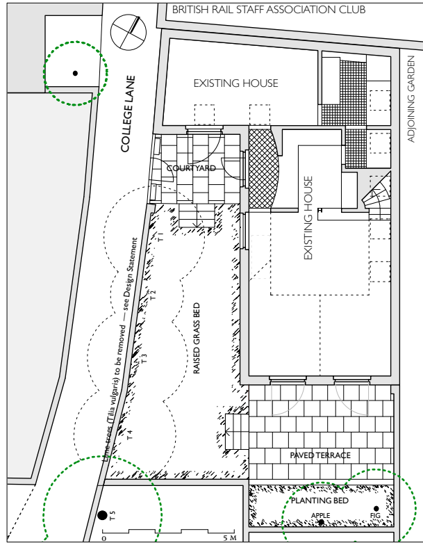
1 : 200 GROUND PLAN AS EXISTING
