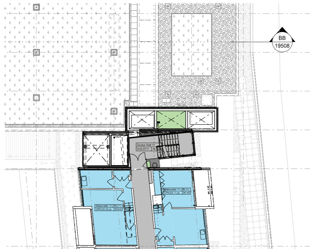
AMENDED PLAN Drawing: 19407-CPA Third Floor Plan
