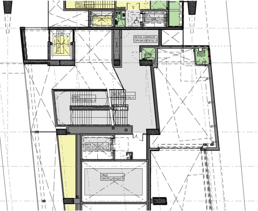
AMENDED PLAN Drawing: 19403-CPA Ground Mezz Floor Plan
