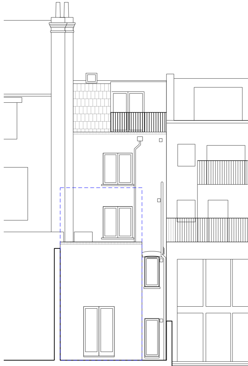
REAR ELEVATION
