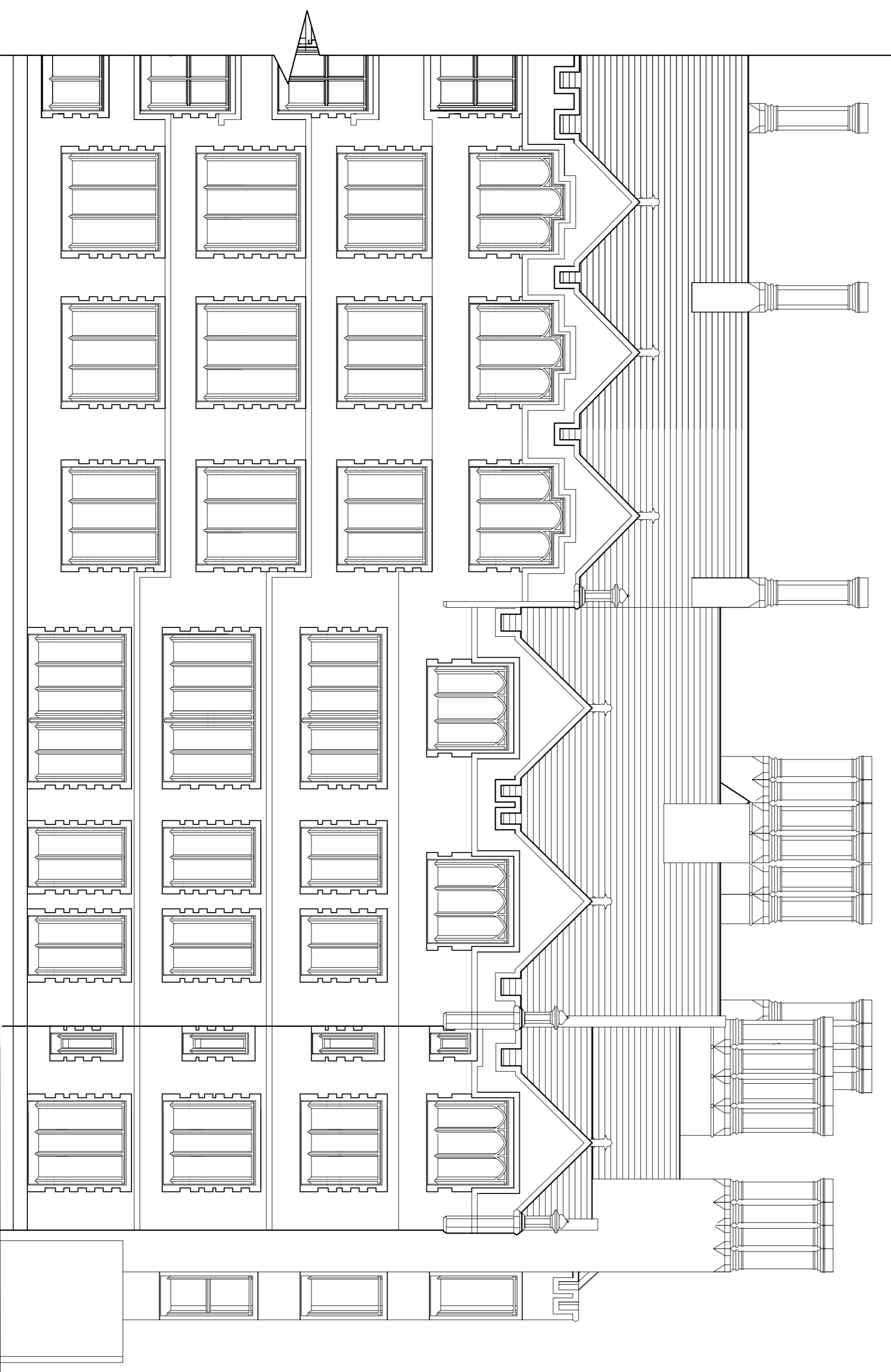
Elevation A Part 1
