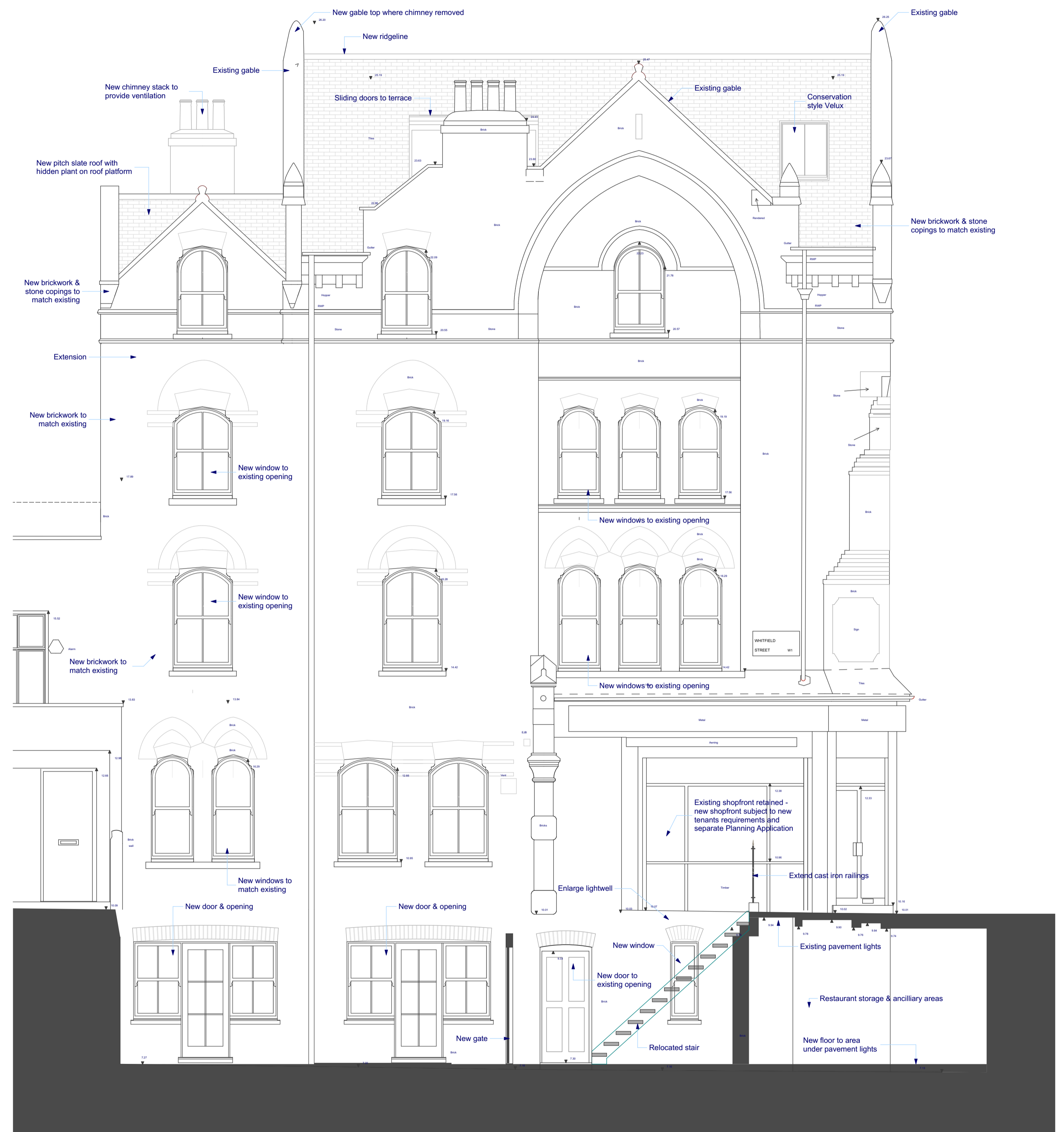
WHITFIELD STREET ELEVATION
