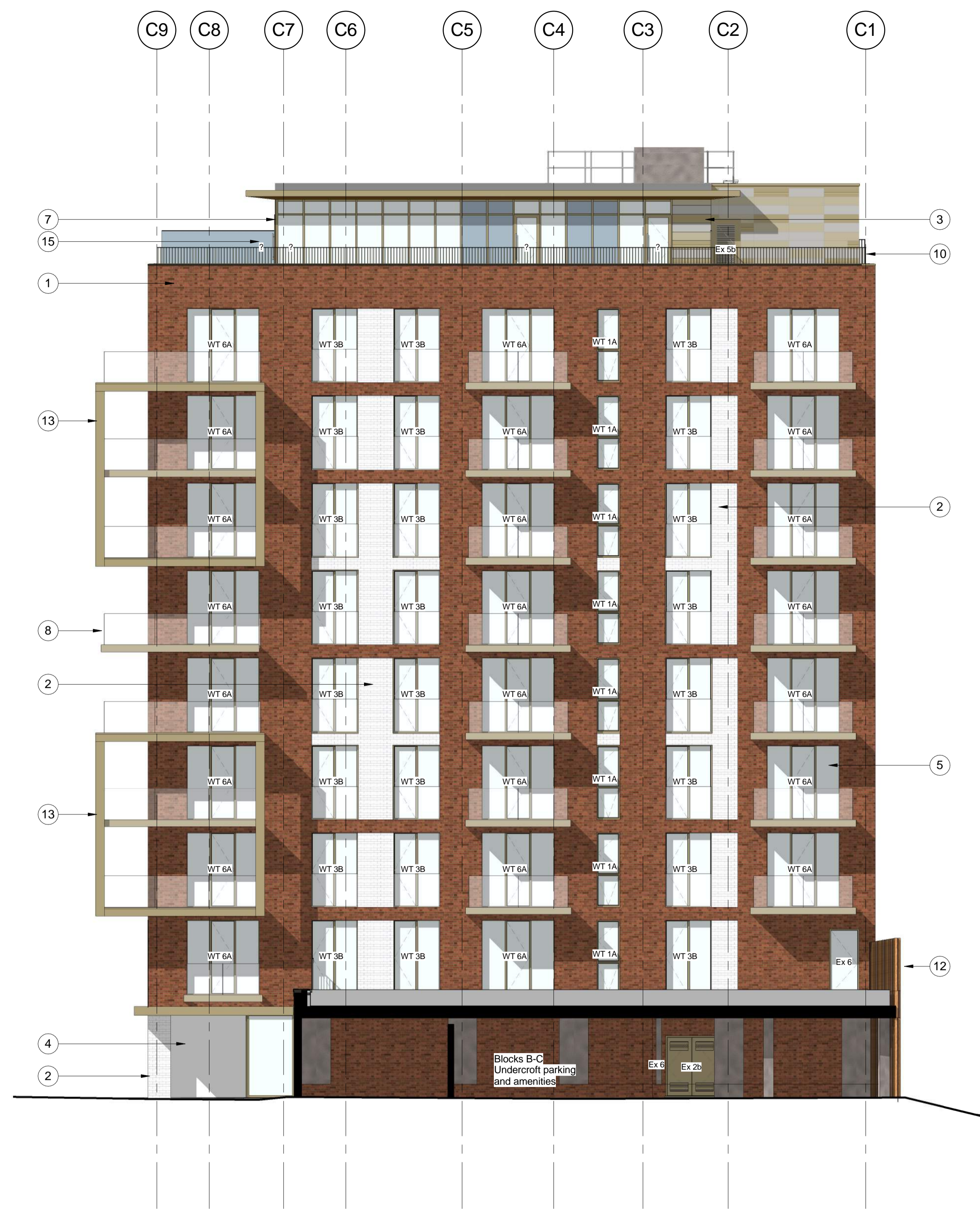
3 Block C East 1 : 100
