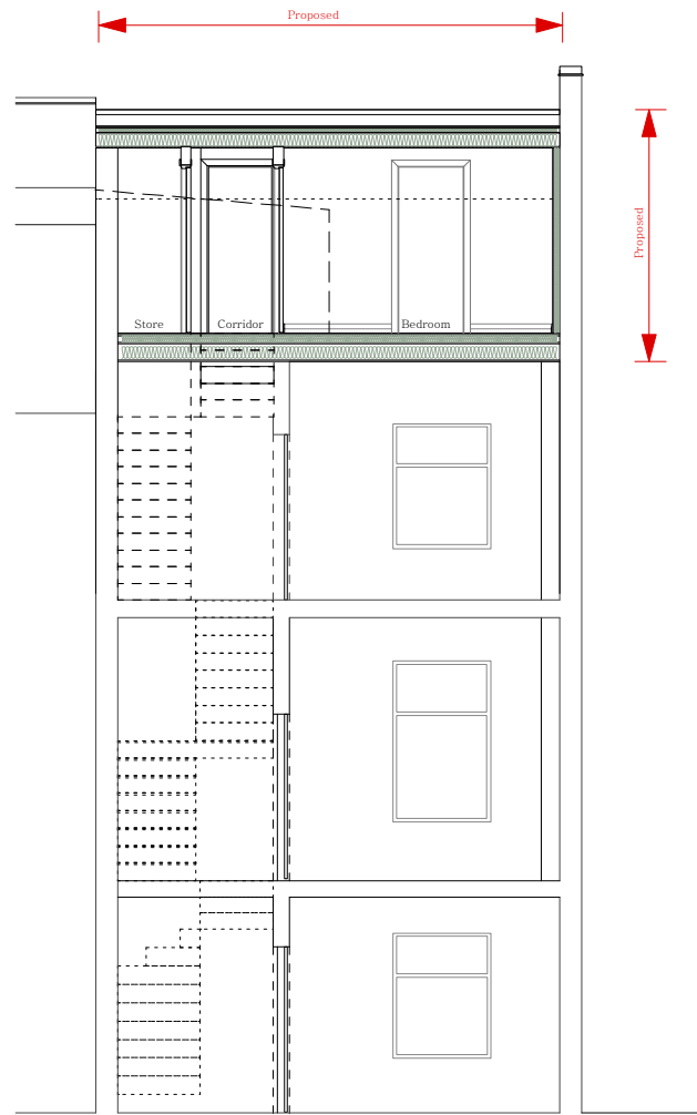
Proposed Section BB
