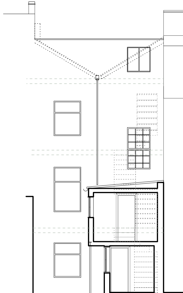
Section BB
