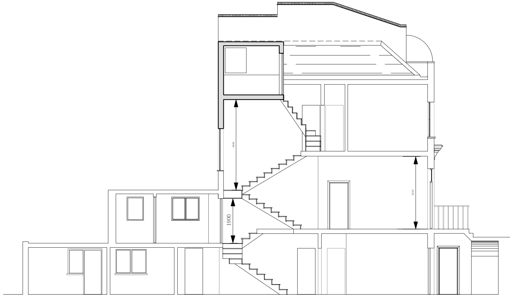
Section AA
