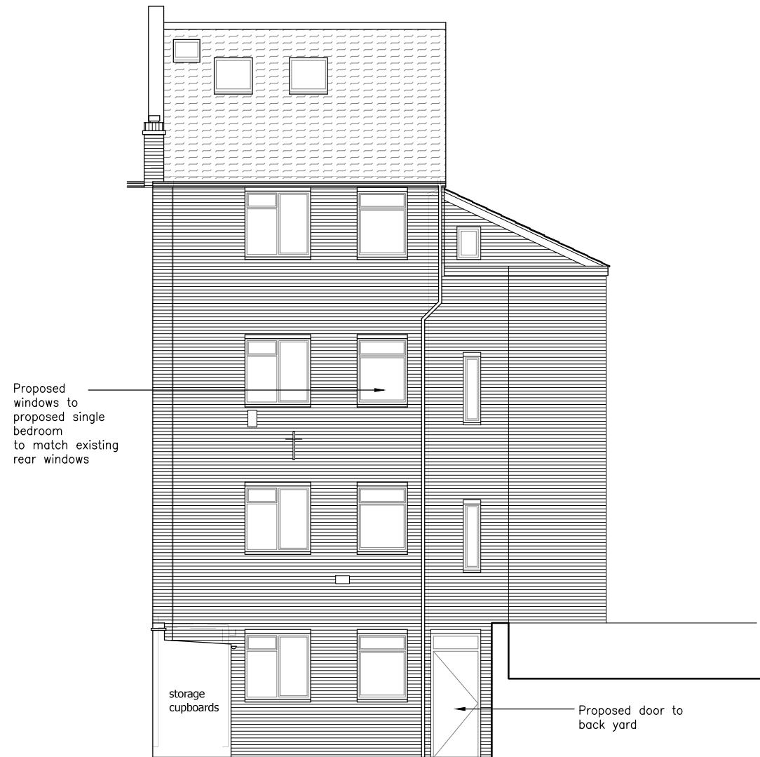
REAR ELEVATION
