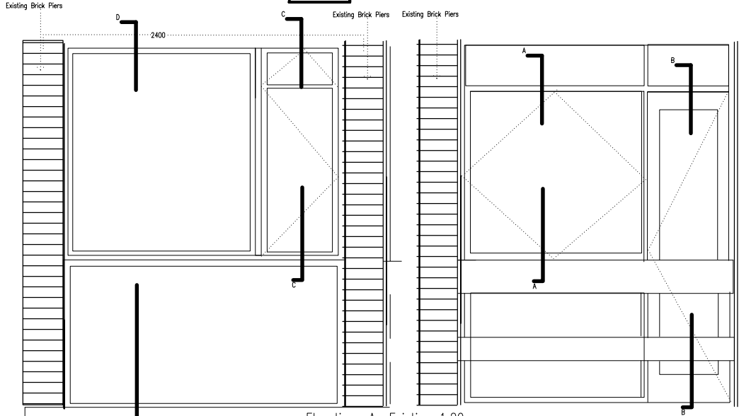
Elevations As Existing 1:20
