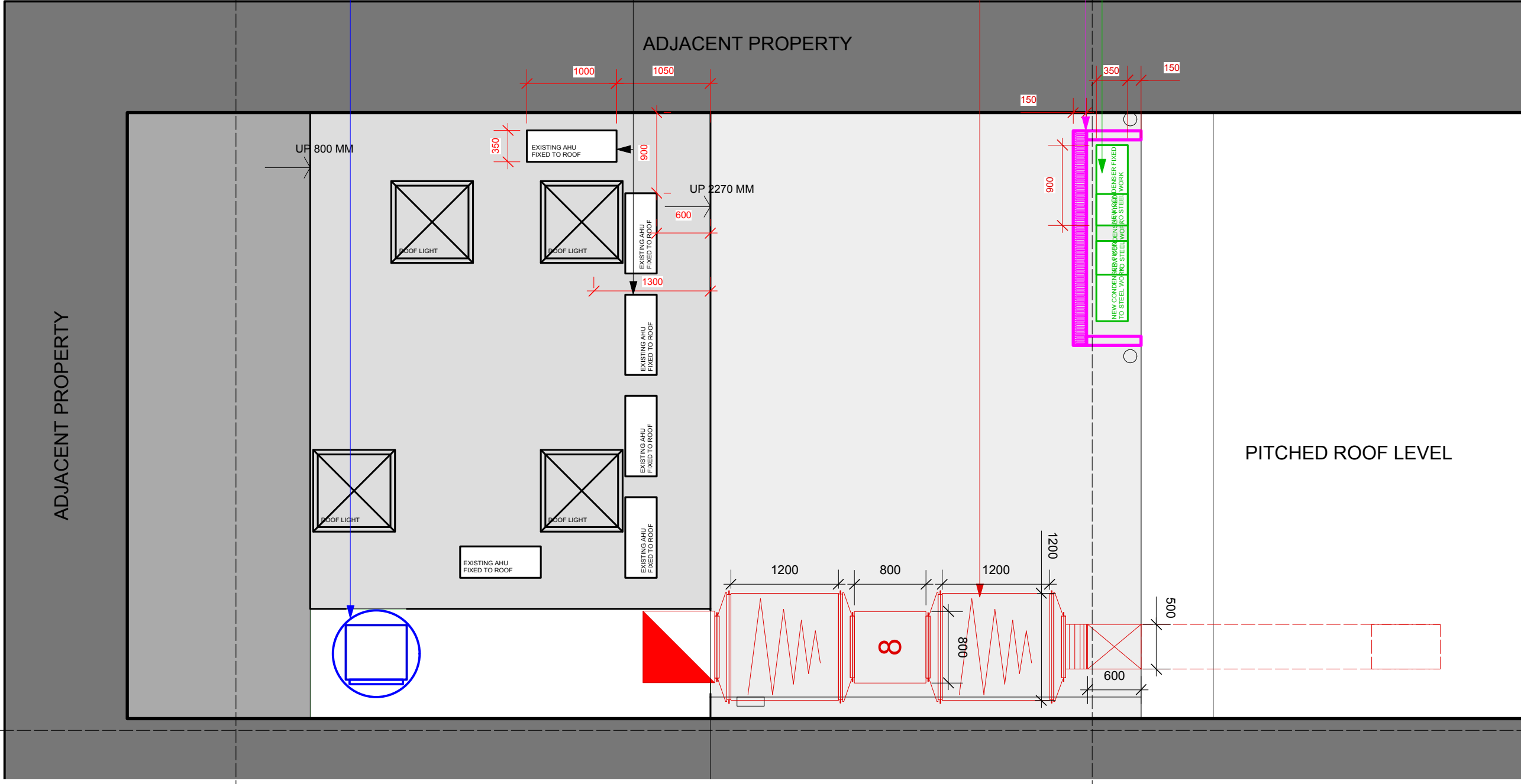
789 - ROOF PLAN SCALE 1:50 @ A3
