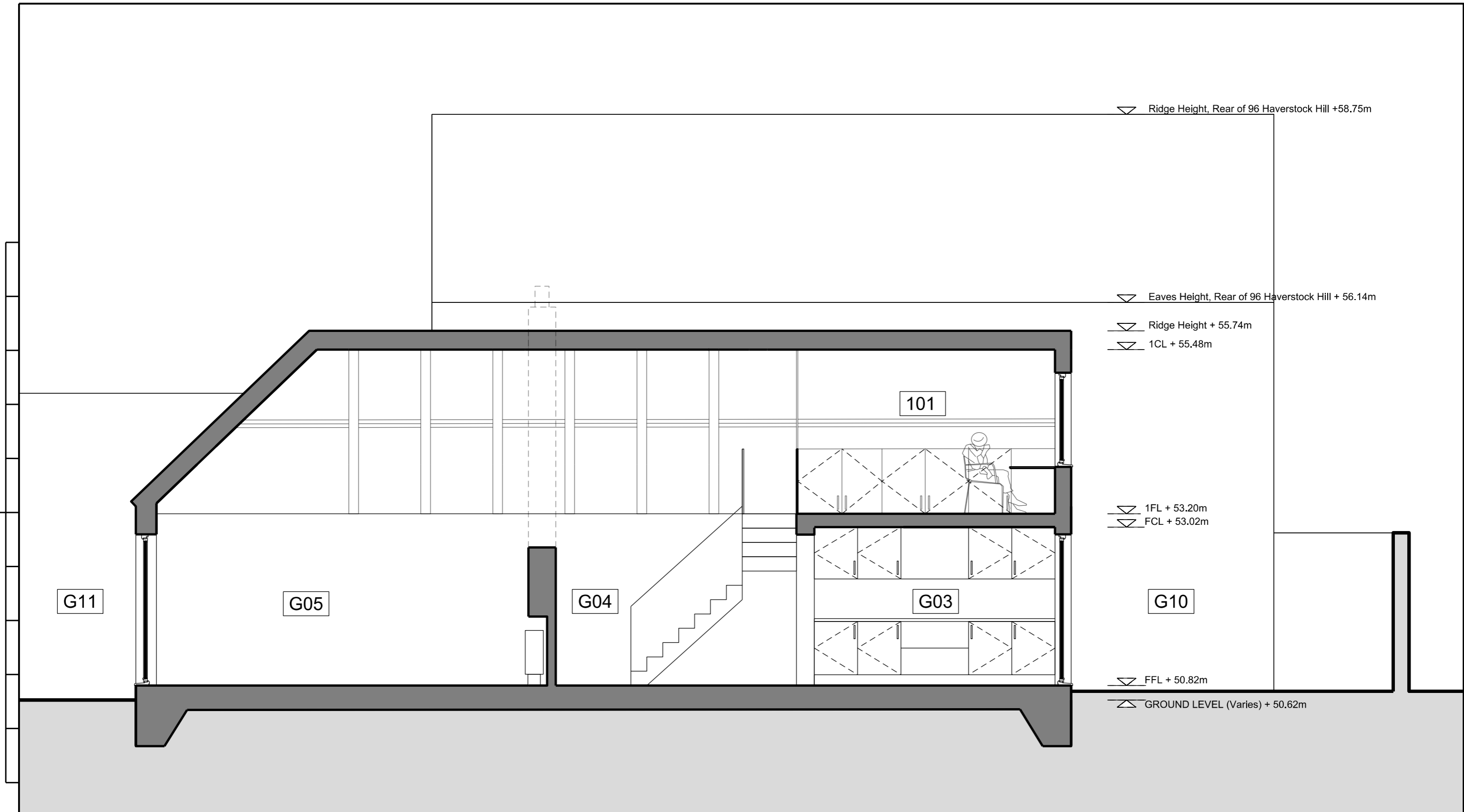
AA 210 Proposed Section BB 1:50
