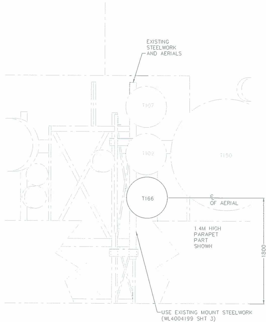
ELEVATION VIEW OF MOUNT 1 FACING 91 DEGREES SCALE 1:15
