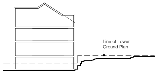
02 PL103 KEY SECTION. 1:500 @A3
