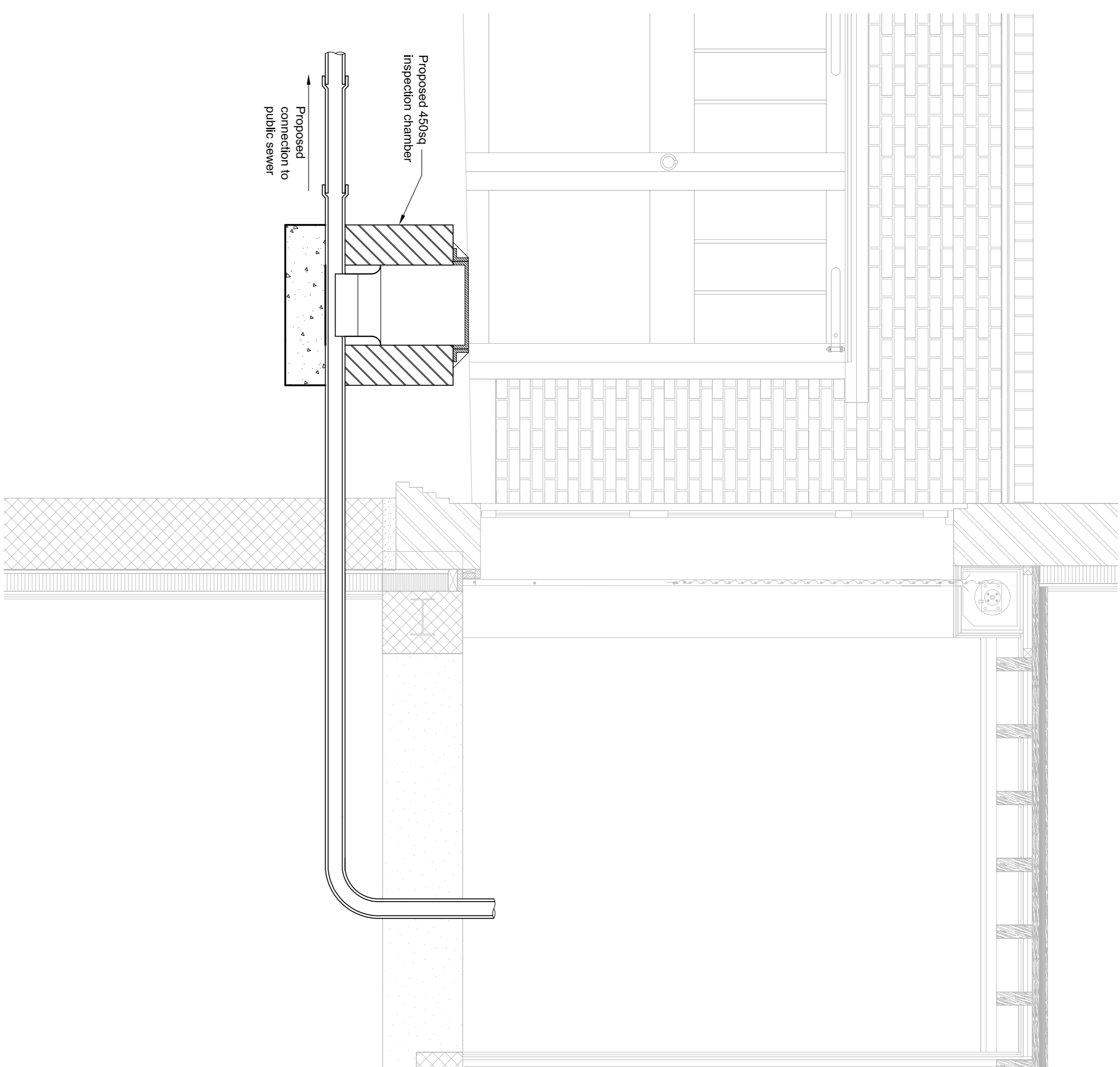
SECTION 1-1 SCALE 1:20
