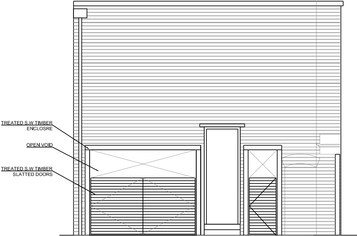
4 A1-103 PROPOSED ELEVATION OF EXTERNAL REFUSE AREA SCALE 1:50 at A3
