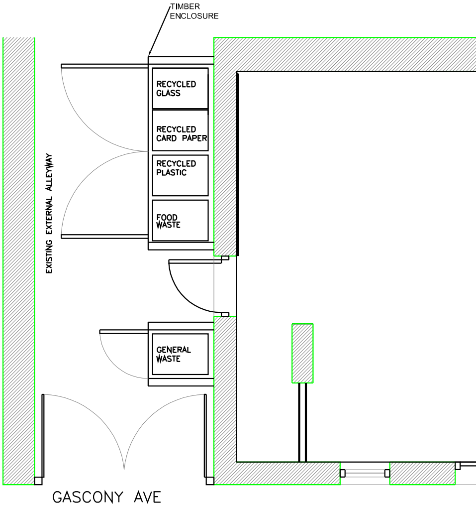
2 A1-103 PROPOSED PLAN OF EXTERNAL REFUSE AREA SCALE 1:50 at A3
