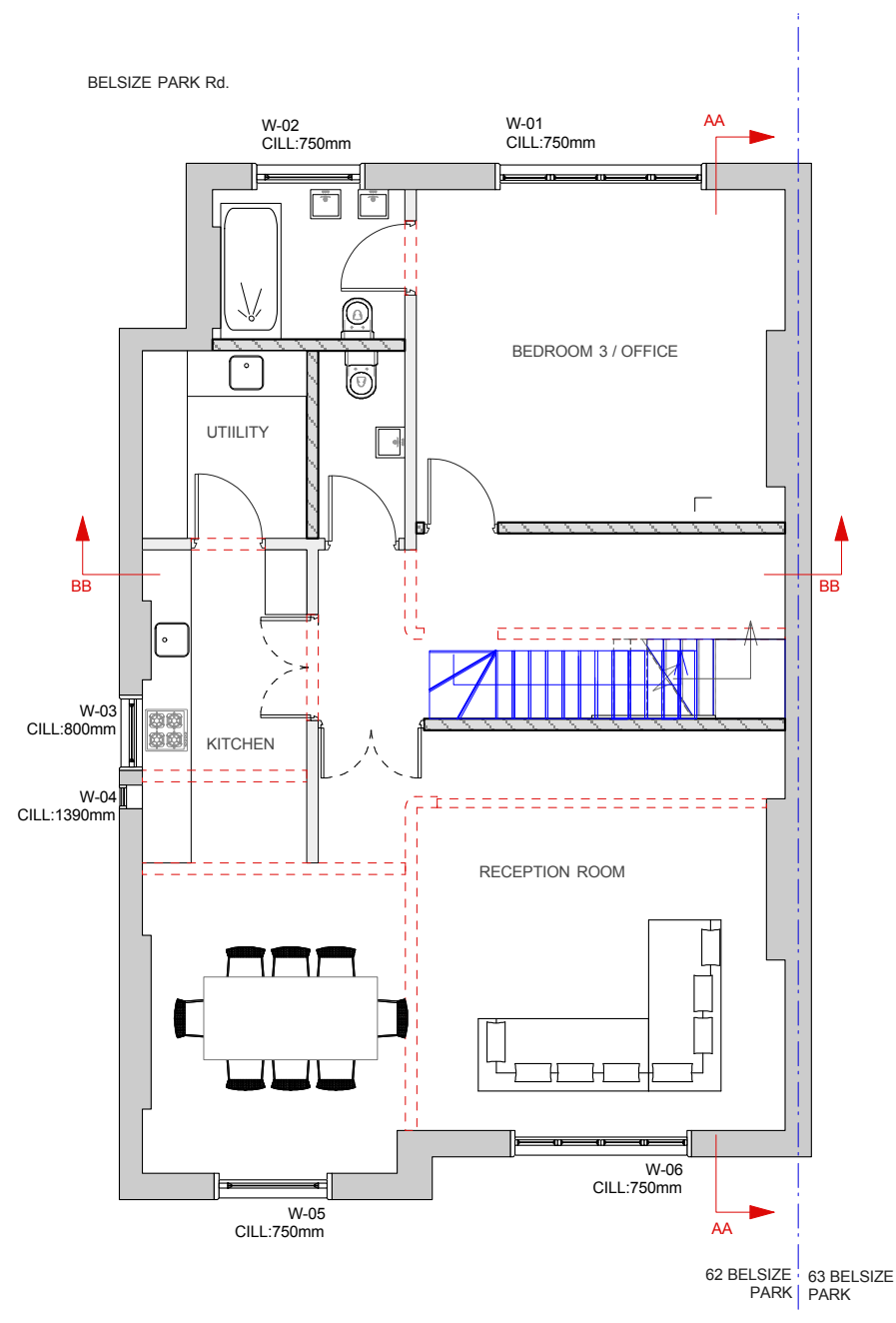
1 62 BELSIZE PPROPOSED SECOND FLOOR Scale: 1:100
