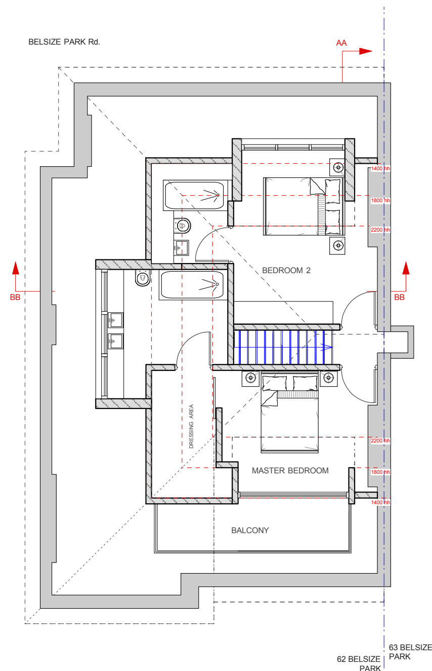
2 62 BELSIZE PARK-PROPOSED LOFT Scale: 1:100
