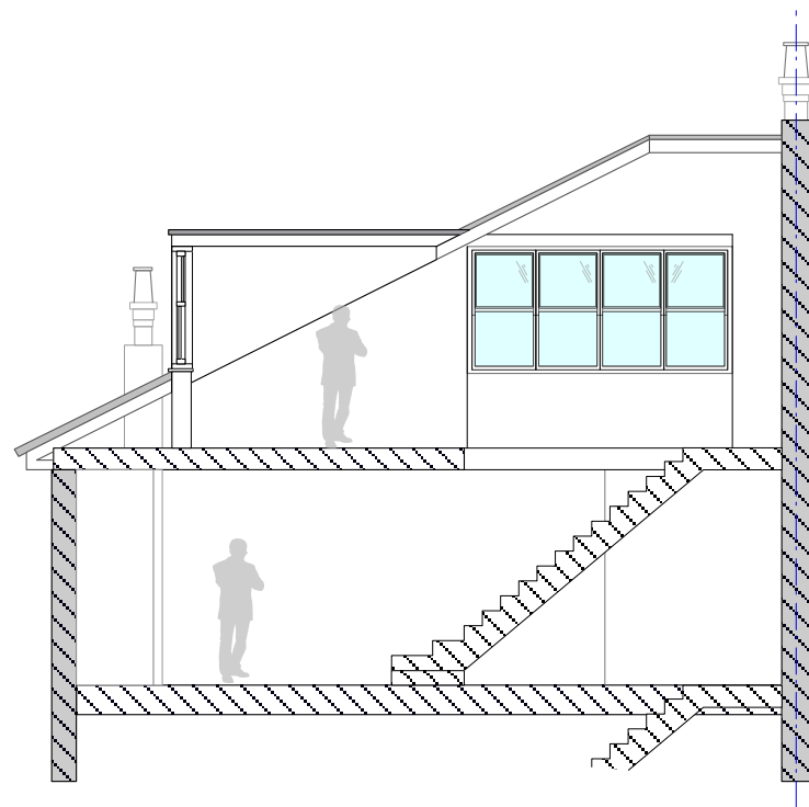
5 62 BELSIZE PARK- PROPOSED SECTION BB Scale: 1:100
