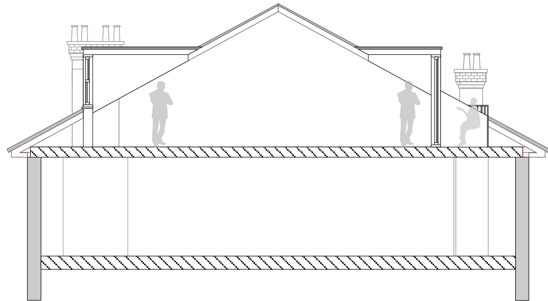
4 62 BELSIZE PARK- PROPOSED SECTION AA Scale: 1:100
