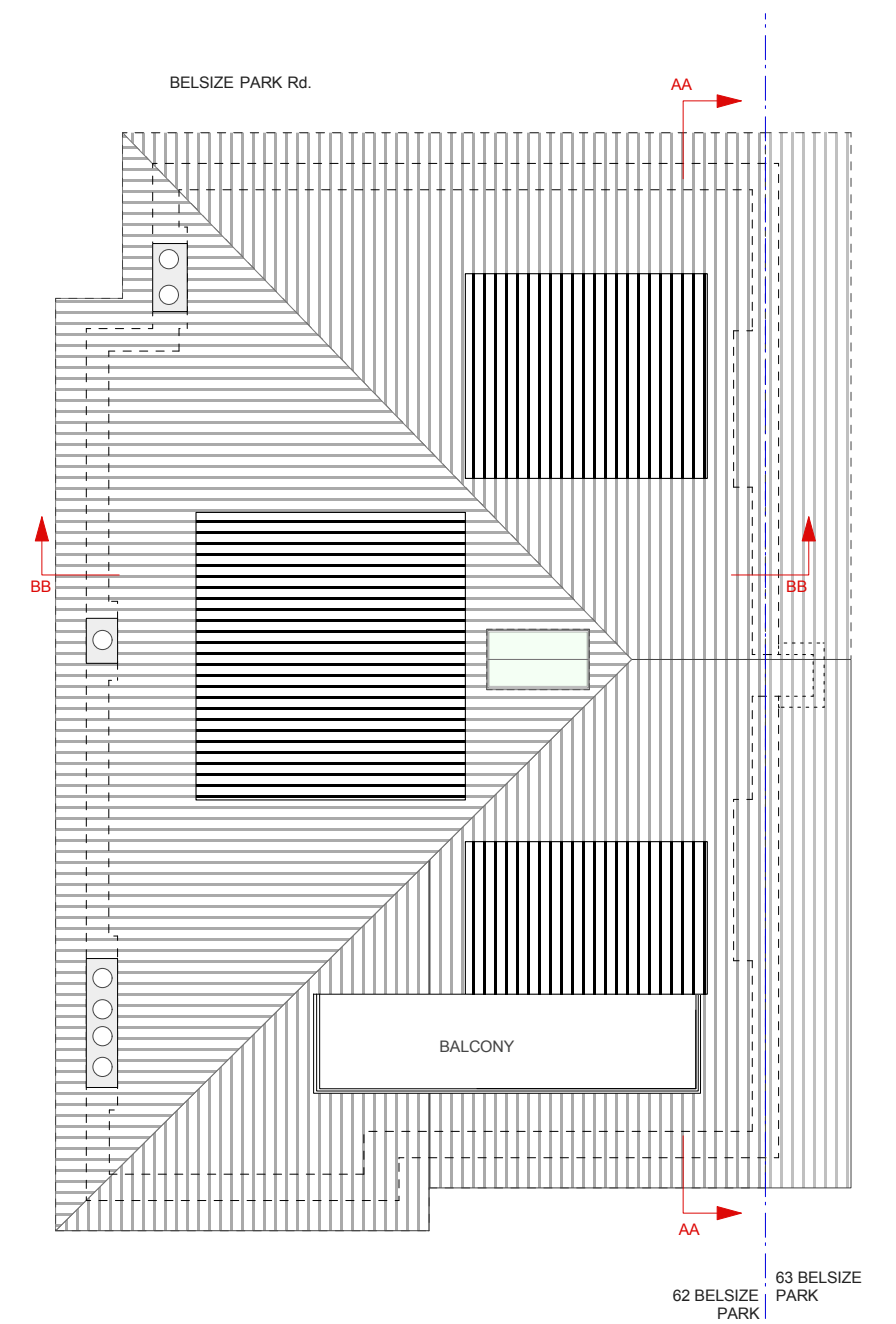
3 62 BELSIZE PARK- PROPOSED ROOF Scale: 1:100
