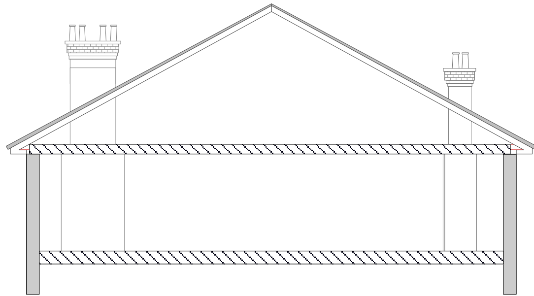
1 62 BELSIZE PARK- EXISTING SECTION AA Scale: 1:100
