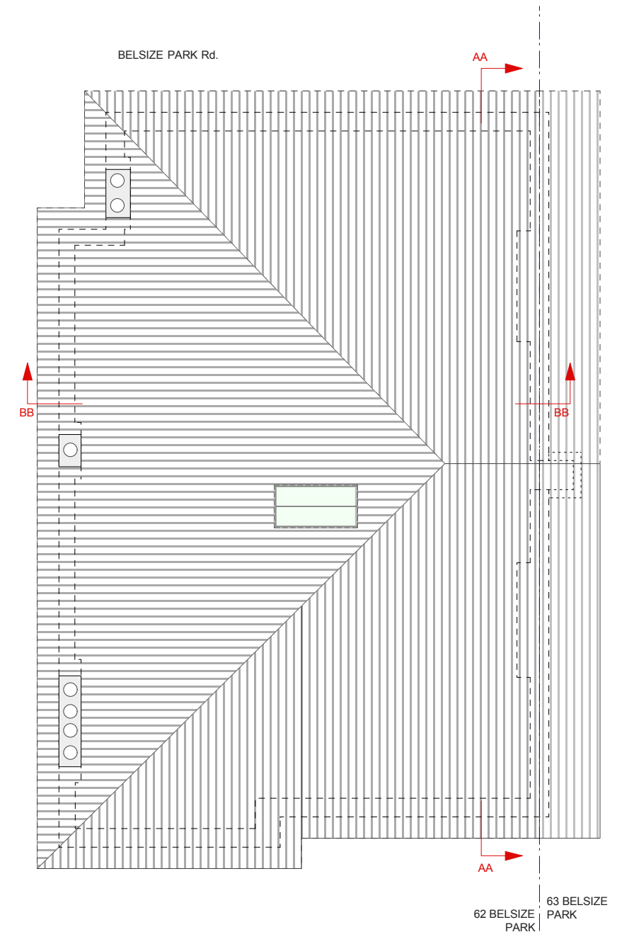
3 62 BELSIZE PARK- EXISTING ROOF Scale: 1:100
