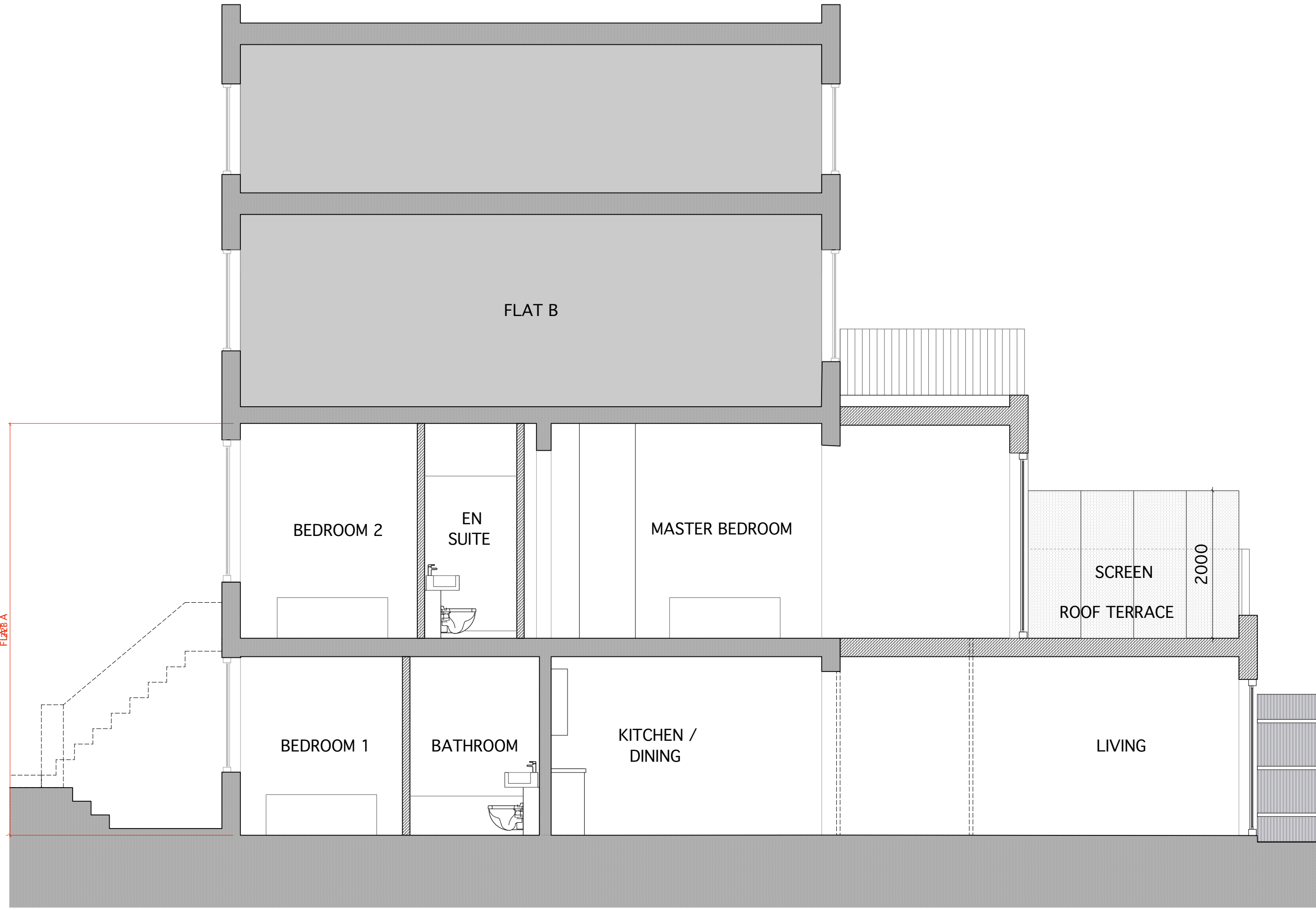
1 PROPOSED SECTION Scale: 1:25
