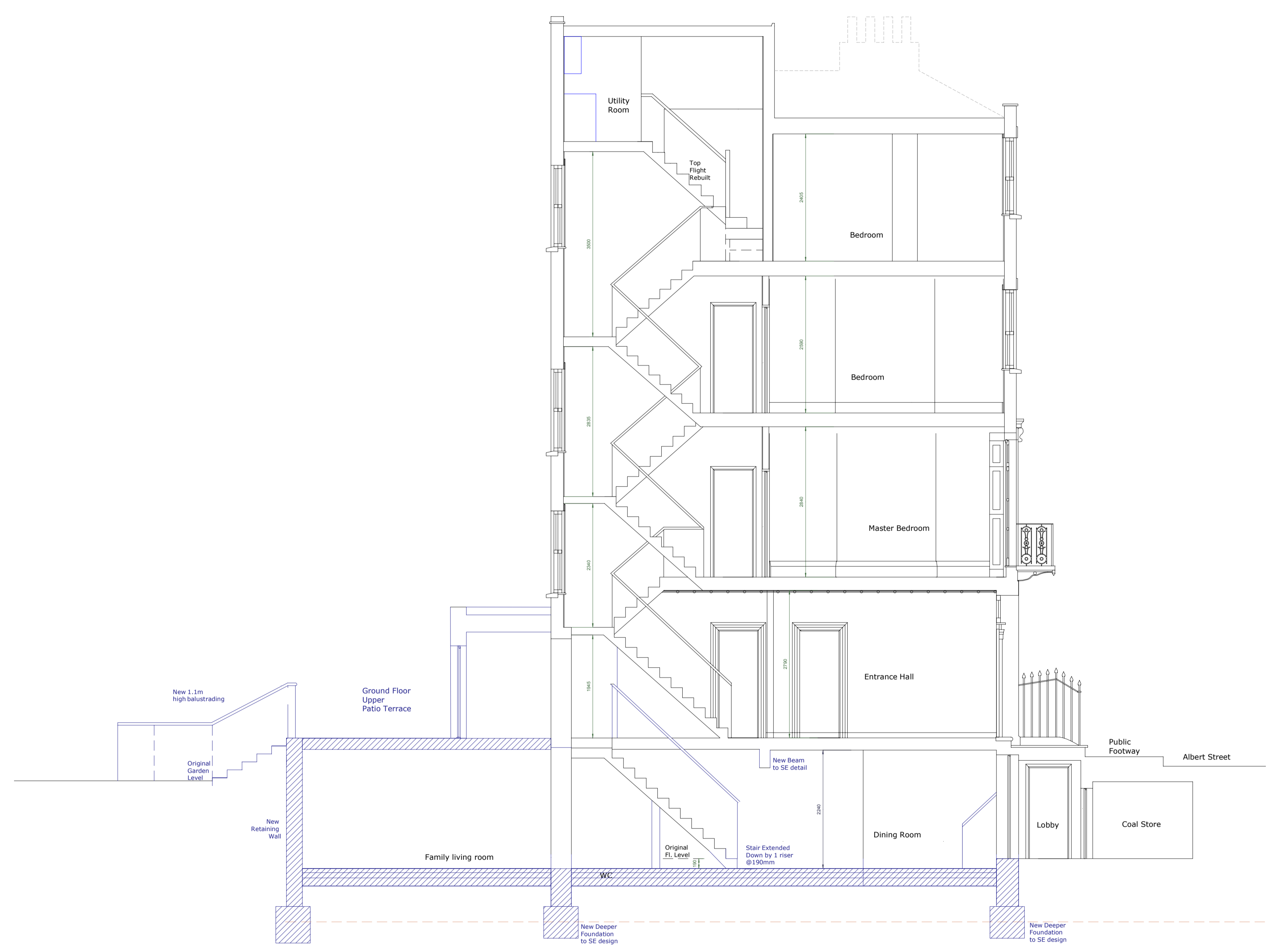
Cross Section A - A' As Proposed
