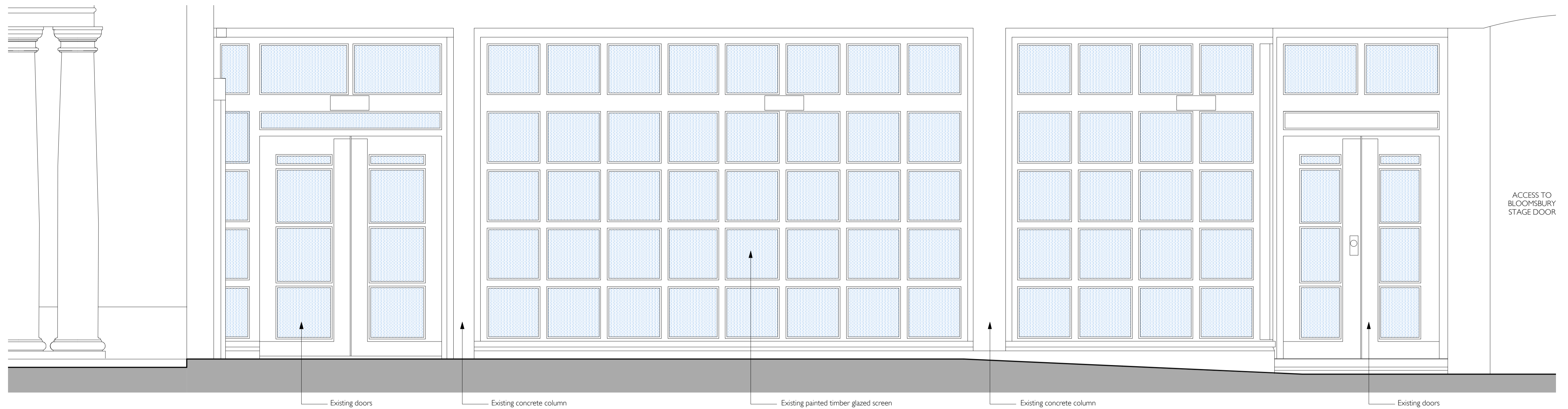
05 Existing Doors / Glazed Screen Detail 05 1:20 @ A1
