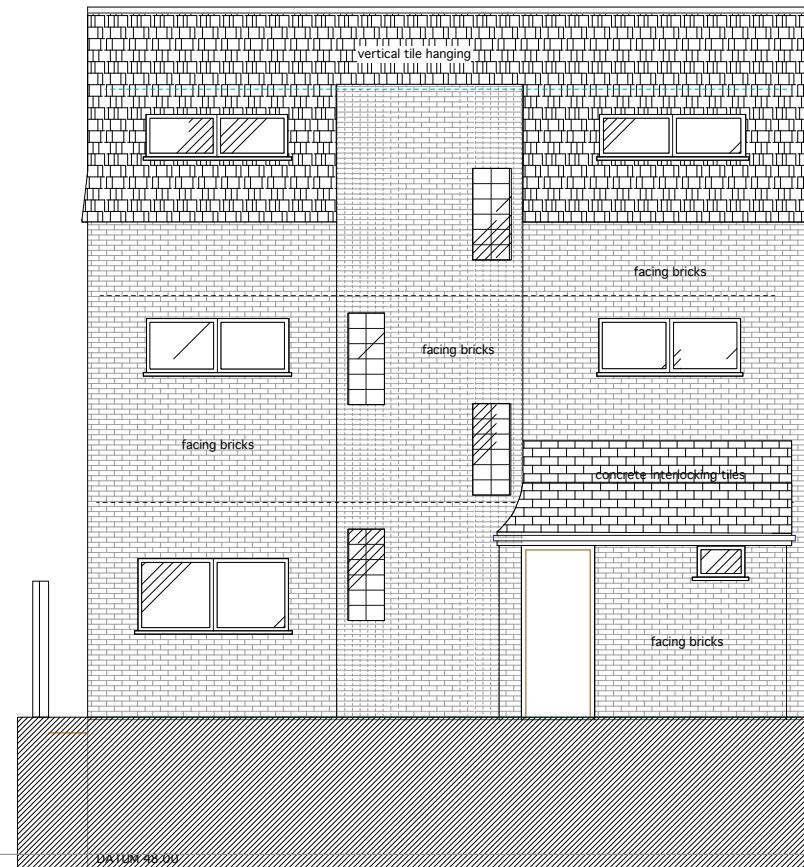
EAST FRONT ELEVATION
