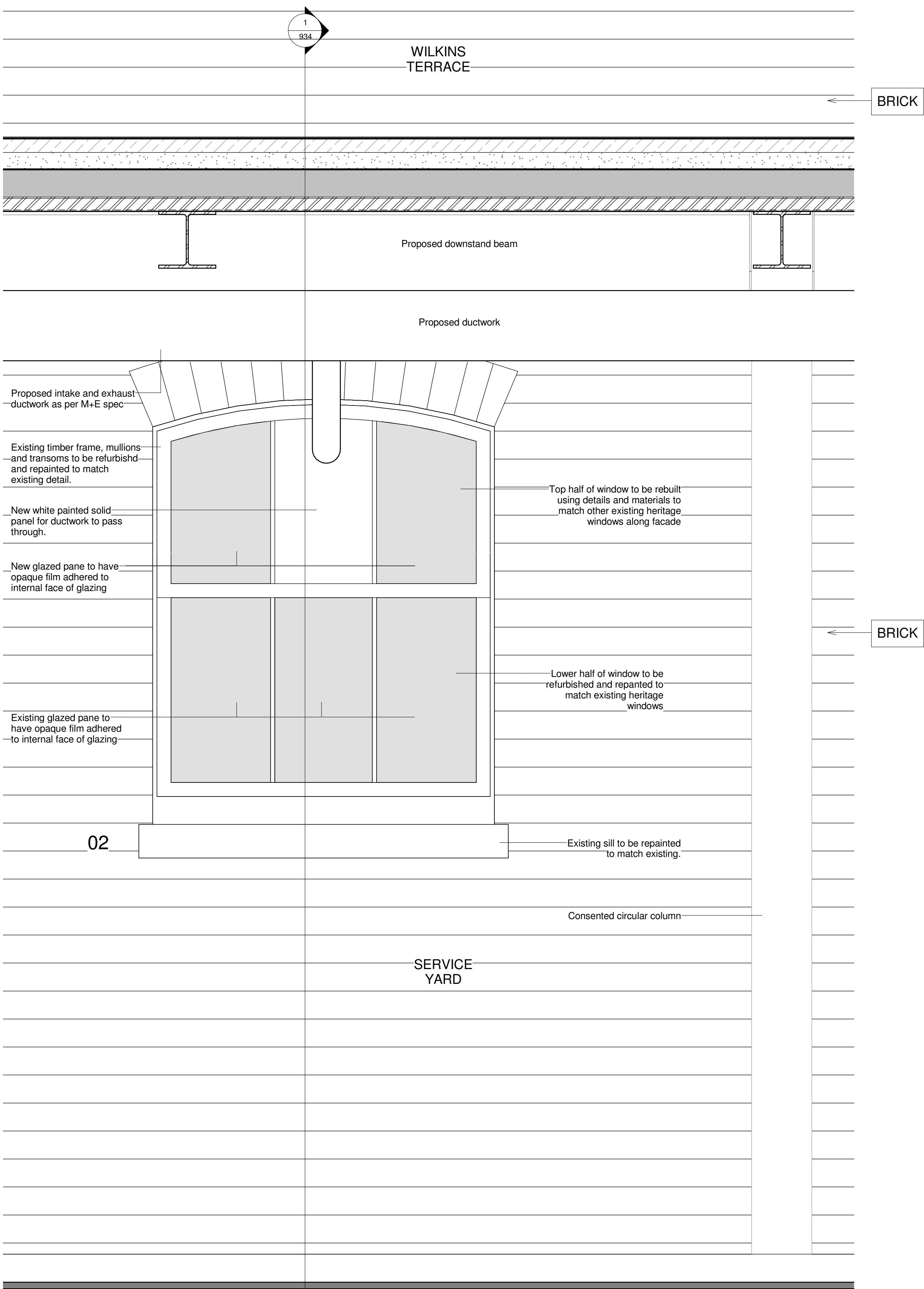
Proposed Heritage Window - Elevation 1 : 10
