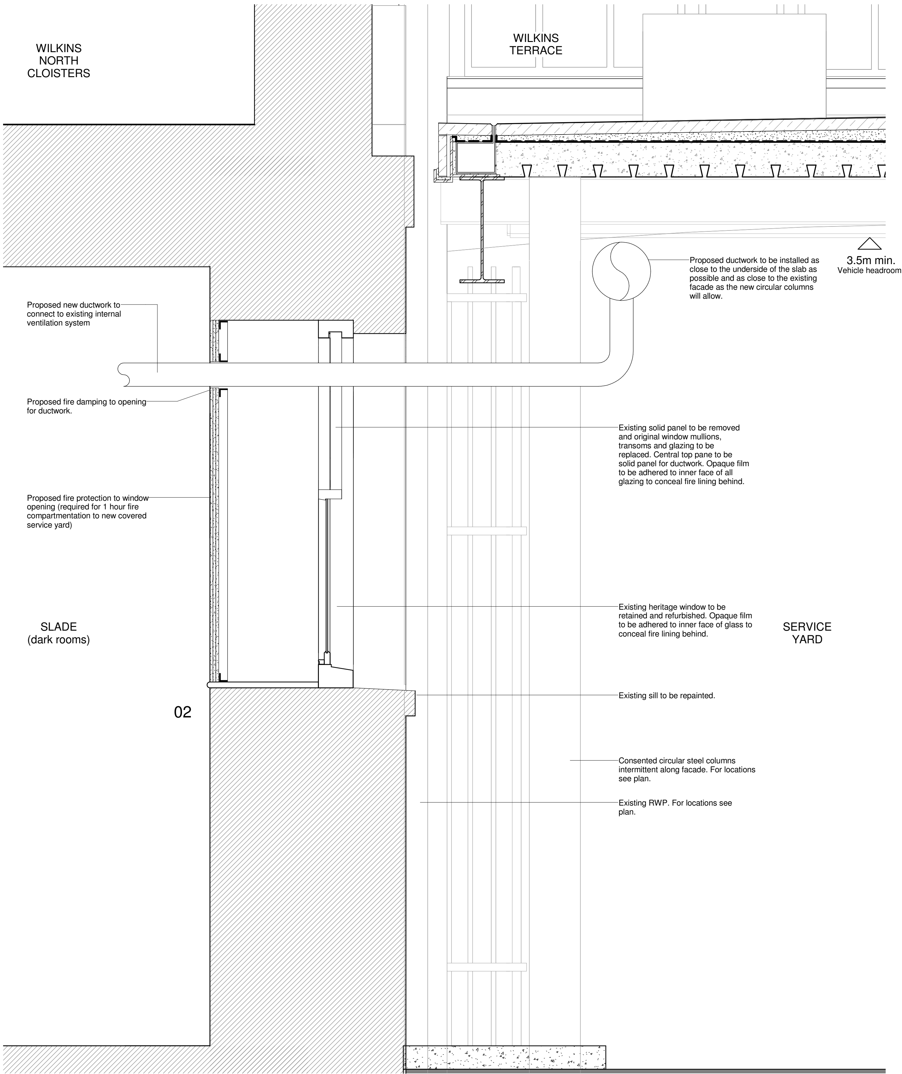
Proposed Alterations to Heritage Windows - Detail Section 1 : 10
