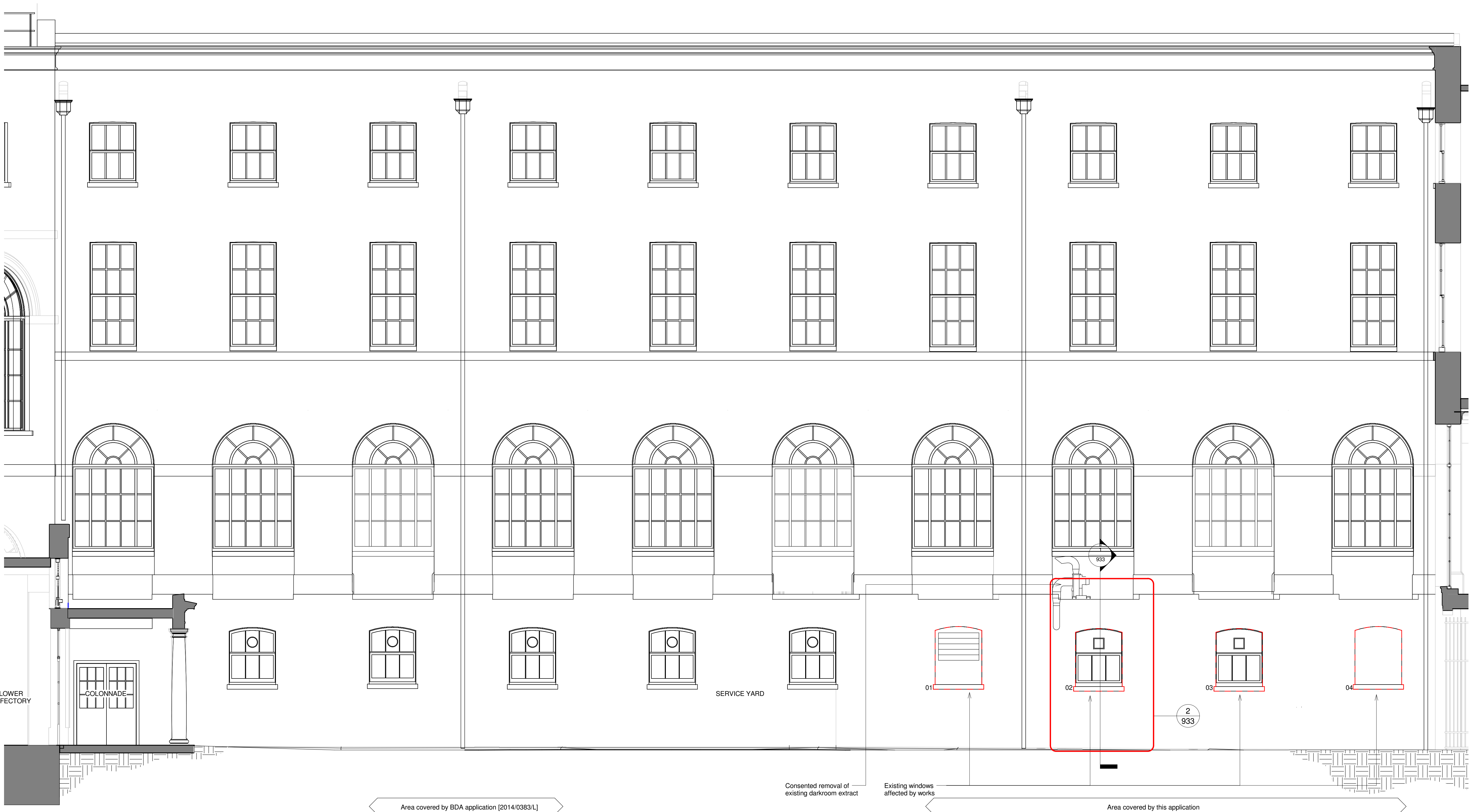
Existing Wilkins North Cloister Elevation 1 : 50
