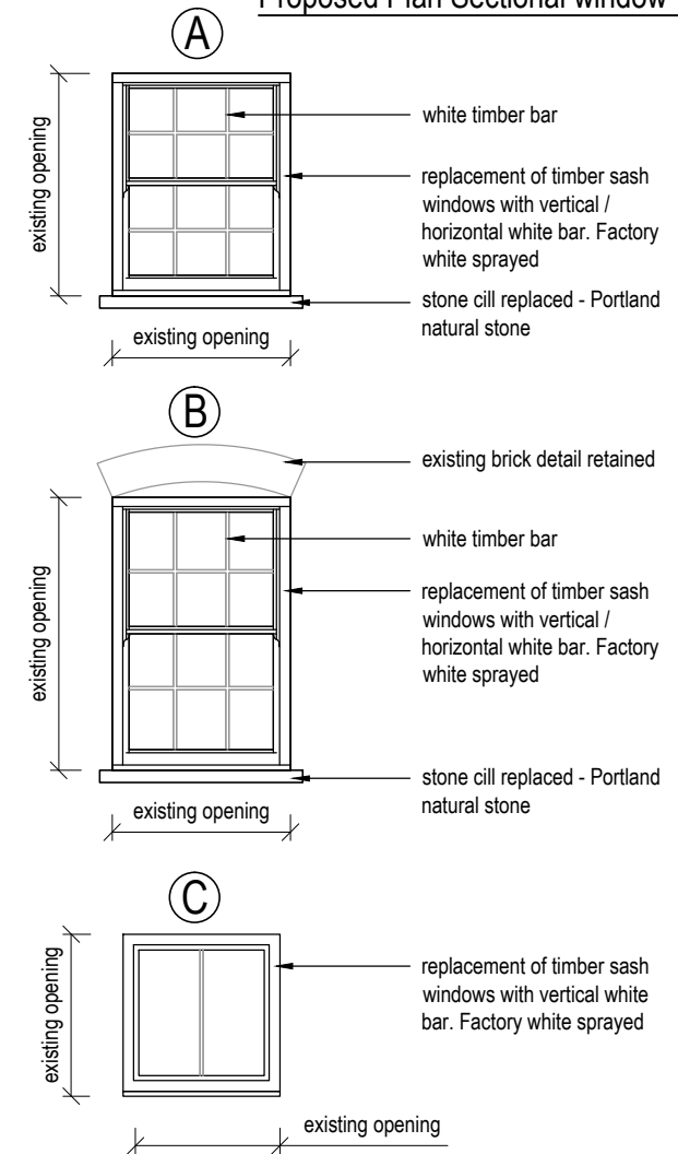
Proposed Plan Sectional window 1:5
