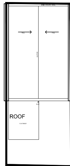
02- EXISTING BLOCK PLAN 1:200
