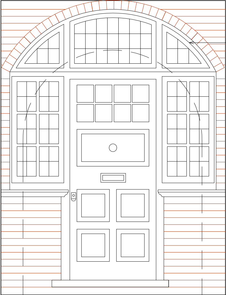
PROPOSED ELEVATION OF MAIN ENTRANCE DOOR 1 : 25
