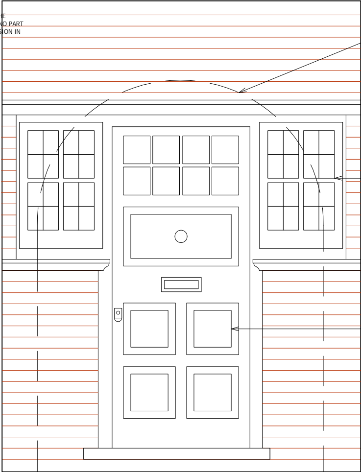
EXISTING ELEVATION OF MAIN ENTRANCE DOOR 1 : 25
