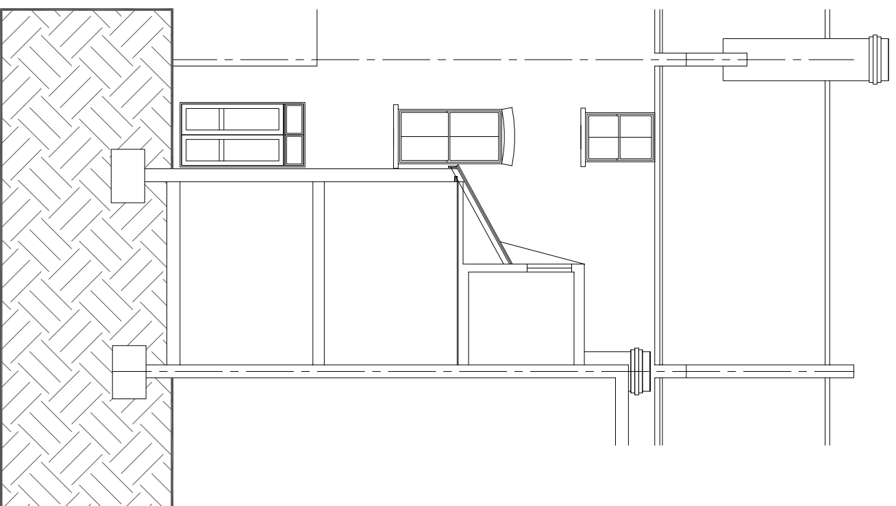
SECTION C
