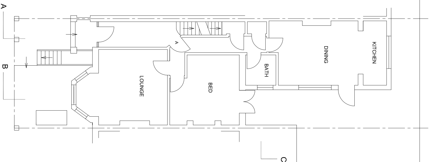
UPPER GROUND FLOOR
